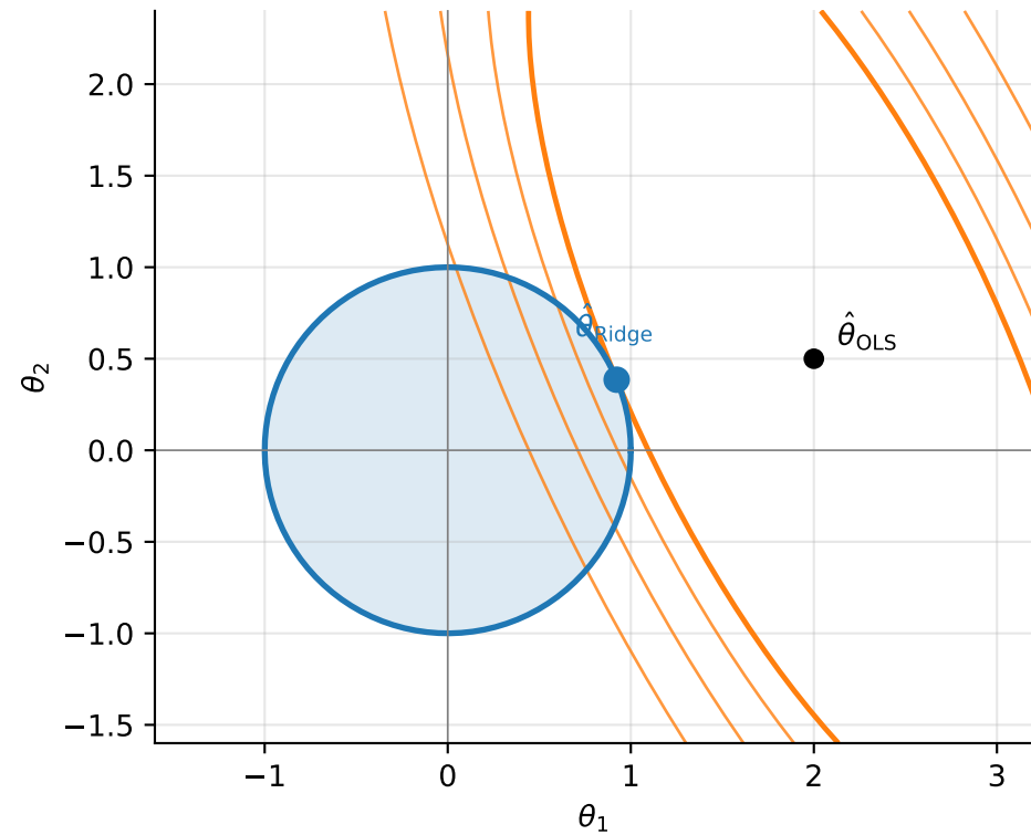
Ridge: \theta_1^2 + \theta_2^2 \leq t
