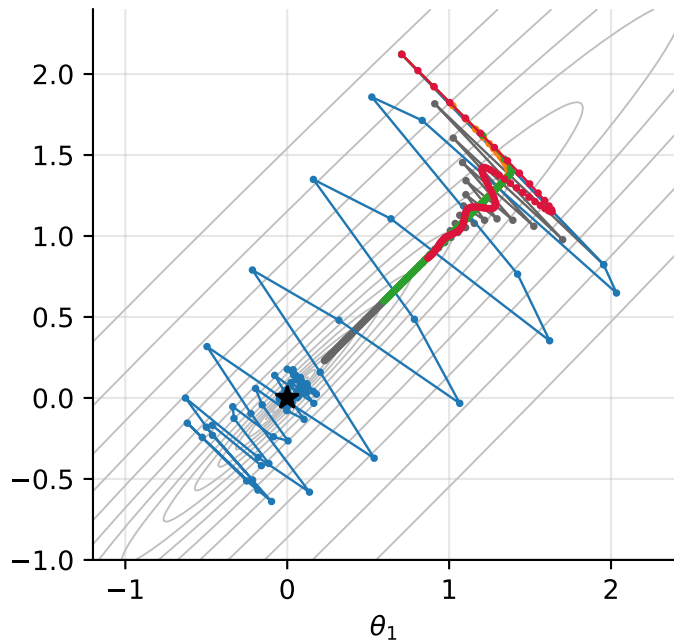
rotated by 45^\circ : \mathbf{H} = \mathbf{Q} \text{diag}(1, 100) \mathbf{Q}^T
