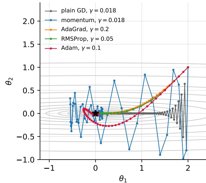
axis-aligned: \mathbf{H} = \text{diag}(1, 100)
