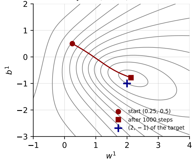
no hidden layer: C(w^1, b^1) and the descent
