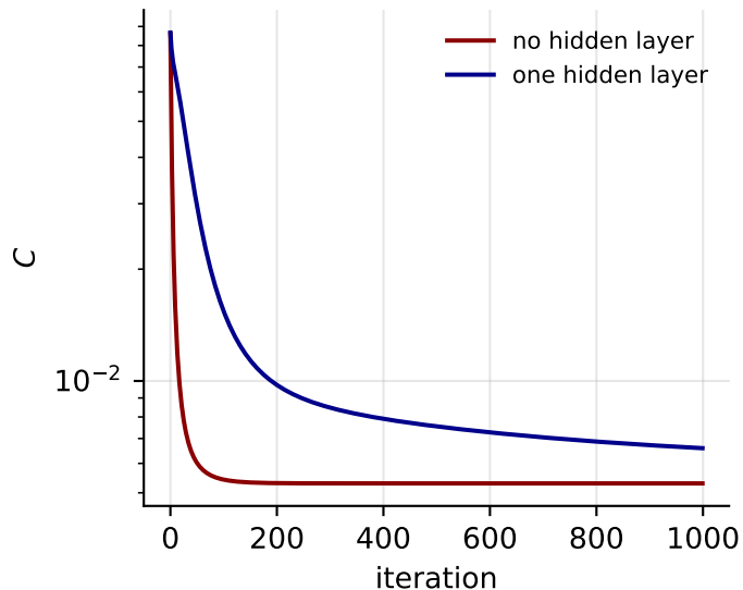
cost, plain gradient descent, \gamma = 2
