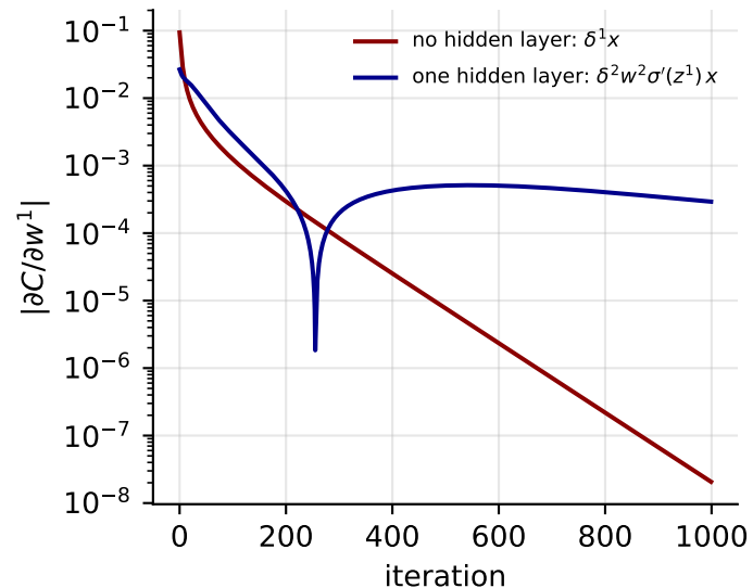
gradient reaching the first weight
