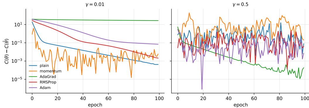
Fig. 4.9 Excess cost against epoch for the five optimisers of Section 4.12 at two learning rates. The vertical axis is C(\theta) minus its value at the analytical minimum. The ranking of the methods reverses between the panels.
