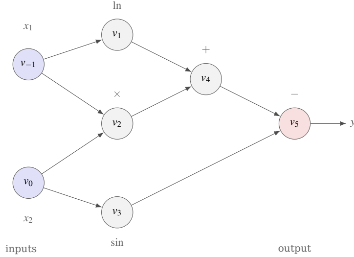
Fig. 4.10 The computational graph of the evaluation trace (4.78) for f(x_1, x_2) = \ln x_1 + x_1 x_2 - \sin x_2 . Each node is one elementary operation applied to its predecessors. Forward-mode AD sweeps this graph from left to right, carrying a derivative \dot{v}_i with every value; reverse-mode AD first evaluates the values from left to right and then sweeps back from right to left, carrying an adjoint \bar{v}_i = \partial y / \partial v_i with every node.
