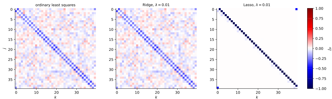
Fig. 3.9 The coupling matrices J_{jk} recovered from 400 configurations of the L = 40 Ising chain. The truth is a single off-diagonal band. OLS and Ridge spread the interaction over the whole matrix and split each coupling symmetrically between (j, k) and (k, j) ; the Lasso finds the band and puts each coupling entirely on one side of the pair. Both behaviours are forced, by Proposition 3.15.
