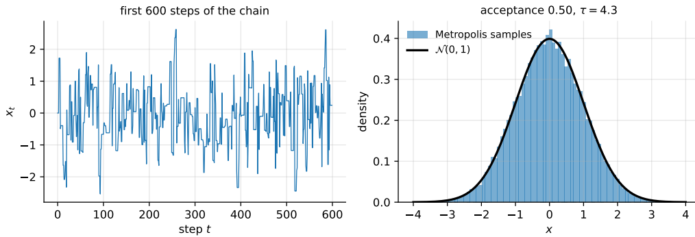
Fig. 2.5 Metropolis sampling of an unnormalised standard Gaussian, Eq. (2.64). Left: the first 600 states of the chain, showing the correlation between successive samples. Right: the sampled histogram against the exact density.
