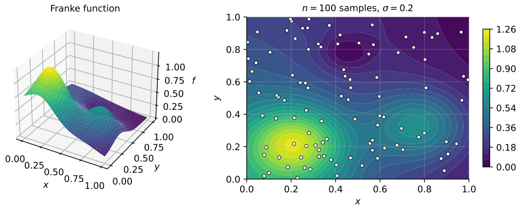
Fig. 3.6 The Franke function (3.100) on the unit square (left) and a contour view with the n = 100 noisy samples used in this section marked (right). Two peaks, a saddle and a depression make it too rich for a low-order polynomial and well within reach of a moderate one.
