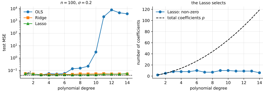
Fig. 3.7 Test error against polynomial degree for the three estimators on the Franke data (left, logarithmic), with the noise floor \sigma^2 = 0.04 marked; and the number of coefficients the Lasso retains against the total number available (right).
