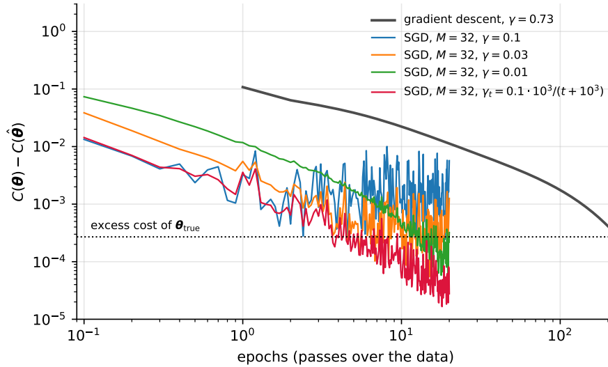
Fig. 5.6 Excess cross entropy C(\boldsymbol{\theta}) - C(\hat{\boldsymbol{\theta}}) against passes over the data for the logistic regression problem of Section 5.9.2 ( n = 50000 , p = 20 , \kappa = 173 ). Gradient descent uses the learning rate (5.46); the SGD runs use minibatches of M = 32 , the cost being recorded ten times per epoch, at three constant learning rates and with the decaying schedule \gamma_t = 0.1 \cdot 10^3 / (t + 10^3) . The dotted line is the excess cost of the parameters that generated the data, about p/(2n) . After a single epoch every SGD run is where gradient descent is after twenty. The constant-rate runs then equilibrate in a cloud whose size grows with \gamma , as Eq. (4.50) predicts, the smallest rate reaching within twenty epochs the level gradient descent needs two hundred for; only the decaying schedule continues downwards.
