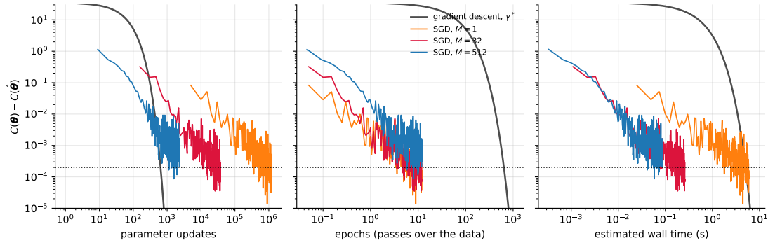
Fig. 4.7 The same four runs – gradient descent at \gamma^* and SGD with M = 1, 32 and 512 and the schedules of Table 4.3 – against three horizontal axes. Left: parameter updates, which favours gradient descent. Centre: epochs, that is, the amount of data processed, on which the three SGD runs coincide. Right: estimated wall time, on which the small batch falls behind. The dotted line is the estimation error \sigma^2 p/n .
