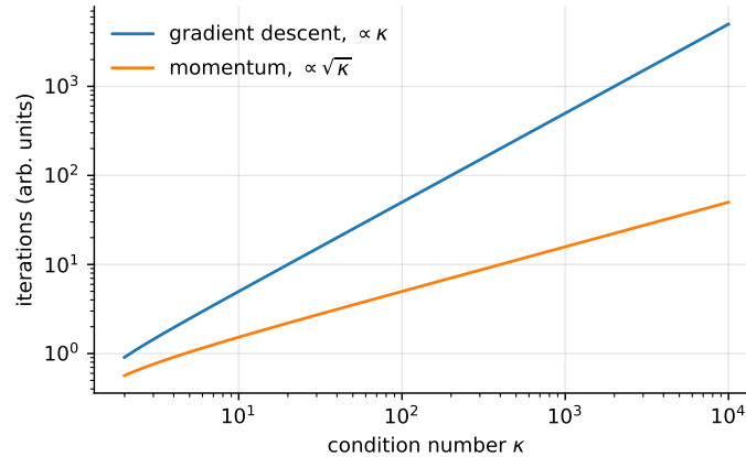
Fig. 4.3 Iterations to fixed accuracy against the condition number, for gradient descent and for momentum with optimal parameters, from the rates (4.26) and (4.33).
