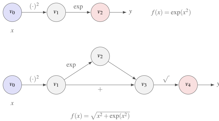
Fig. 4.11 The computational graphs of the two examples of Section 4.14.5. Top: f(x) = \exp(x^2) , trace (4.91), a chain in which every value is used once. Bottom: f(x) = \sqrt{x^2 + \exp(x^2)} , trace (4.95), where v_1 = x^2 feeds both the exponential and the sum. The two paths from v_1 to y are the two terms of the adjoint \bar{v}_1 in Eq. (4.97).
