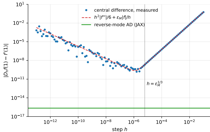
Fig. 4.12 Absolute error of the central finite difference (4.73) for f(x) = \sin(2\pi x + x^2) at x = 1 , as a function of the step h (points), together with the model (4.75) (dashed): truncation error \propto h^2 on the right, rounding error \propto 1/h on the left, and a minimum of about 10^{-10} near h \approx \varepsilon_M^{1/3} . The reverse-mode derivative computed by JAX has an error at the level of the unit roundoff, shown as the horizontal line, for any h because it involves no h .
