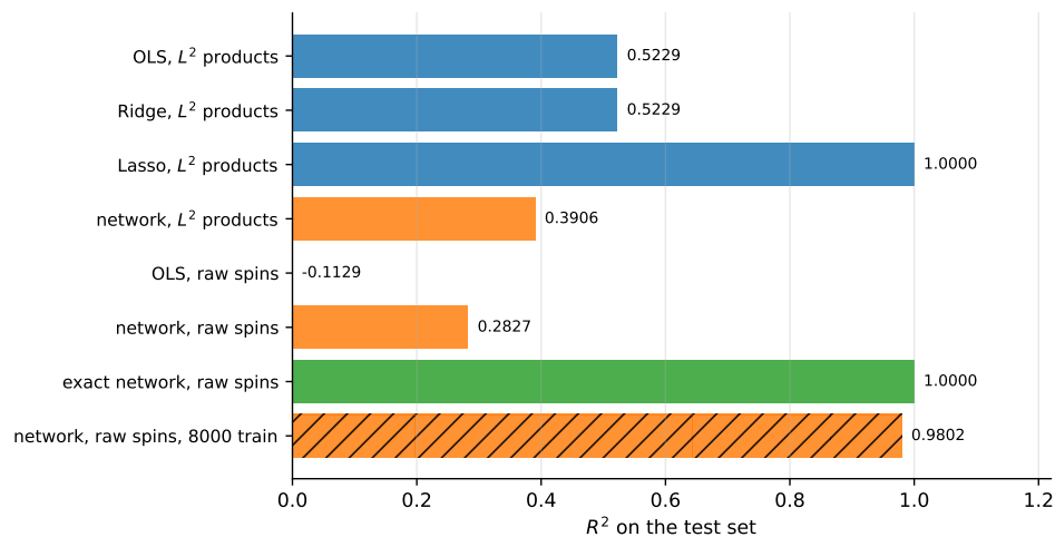
Fig. 8.17 Every model of Section 3.16 and this section on the same problem. Blue: linear models. Orange: trained networks. Green: the exact network of Proposition 8.8. All bars use 400 training configurations and the same 9600 test configurations except the hatched one, which uses 8000 training configurations and a separate held-out set of 2000. Negative scores are drawn as zero and labelled.
