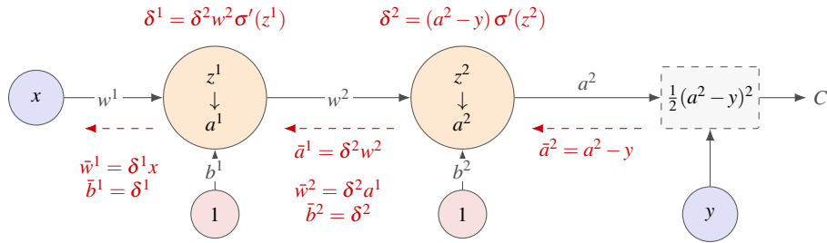
Fig. 8.10 The two scalar networks of Section 8.8.1, drawn in the style of Figure 5.4. Black arrows are the forward pass: each neuron forms z^l = w^l a^{l-1} + b^l from its input and its bias (the weight of an input fixed at one) and emits a^l = \sigma(z^l) ; the dashed box is the squared-error loss. Red dashed arrows are the reverse sweep: the adjoint of the cost is one, it becomes the residual a^L - y at the loss node, the error \delta^L = z^L after the activation, and is then multiplied by whatever sits on the edge it travels along – the input x or a^1 to reach a weight, the constant 1 to reach a bias, and the weight w^2 to reach the hidden neuron, where a further factor \sigma'(z^1) produces \delta^1 . The bottom panel is Eq. (8.43); with several nodes per layer the single edge w^2 becomes the sum over k in Eq. (8.64).
