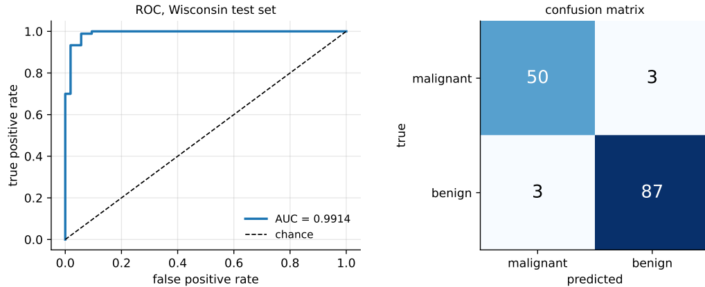
Fig. 5.10 Logistic regression on the Wisconsin test set. Left: the ROC curve, with AUC = 0.9914 . Right: the confusion matrix, whose off-diagonal entries are the two kinds of error and are not equally costly.
