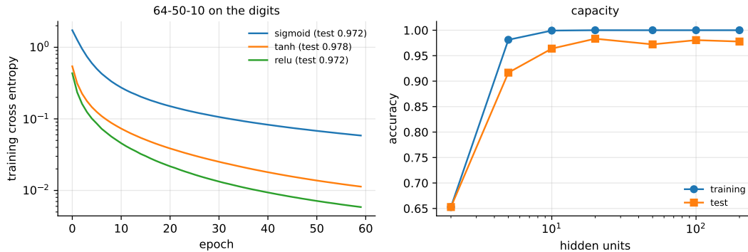
Fig. 8.15 Left: training cross entropy against epoch for three hidden activations on the digits data, with the resulting test accuracies. Right: training and test accuracy against the width of the single hidden layer.
