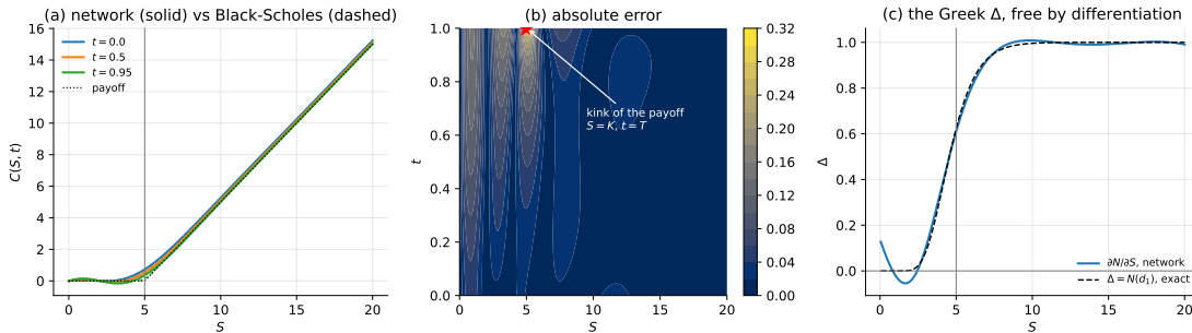
Fig. 9.6 Black-Scholes by a physics-informed network. (a) The option price at three times, network solid and Eq. (9.49) dashed, with the terminal payoff (9.46) dotted; the vertical line is the strike. (b) Absolute error over the whole domain, peaking at the starred point S = K , t = T where the payoff has its kink and the exact solution is not differentiable. (c) The hedge ratio \Delta = \partial C / \partial S obtained by differentiating the trained network, against the exact N(d_1) . The network reproduces it without having been asked to, but goes slightly negative near S = 2 , which no true option price can do.
