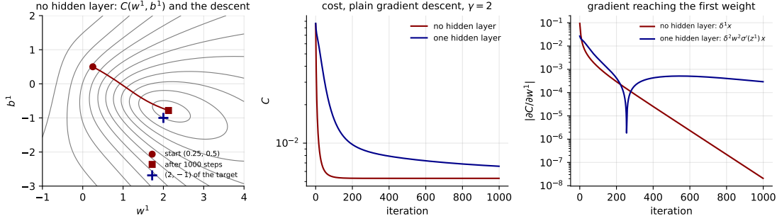
Fig. 8.11 The two scalar networks of Figure 8.10 trained by plain gradient descent, Eq. (8.37), on n = 20 scalar observations y_i = \sigma(2x_i - 1) + \varepsilon_i with \gamma = 2 and 1000 iterations, starting from w^1 = 0.25 , b^1 = 0.5 (and w^2 = 1 , b^2 = -0.5 for the hidden-layer network). Left: the cost surface C(w^1, b^1) of the single neuron and the descent path from the starting point (circle) to its end (square); the cross marks the parameters used to generate the targets. Middle: the cost against iteration for both networks. Right: the magnitude of the gradient reaching the first weight, \delta^1 x in both cases, but with \delta^1 = \delta^2 w^2 \sigma'(z^1) in the deeper network, Eq. (8.43); the extra factor w^2 \sigma'(z^2) attenuates the signal that trains the hidden neuron, a first glimpse of Section 8.9. Generated by BookFigures/ch08_scalar_backprop_figures.py.
