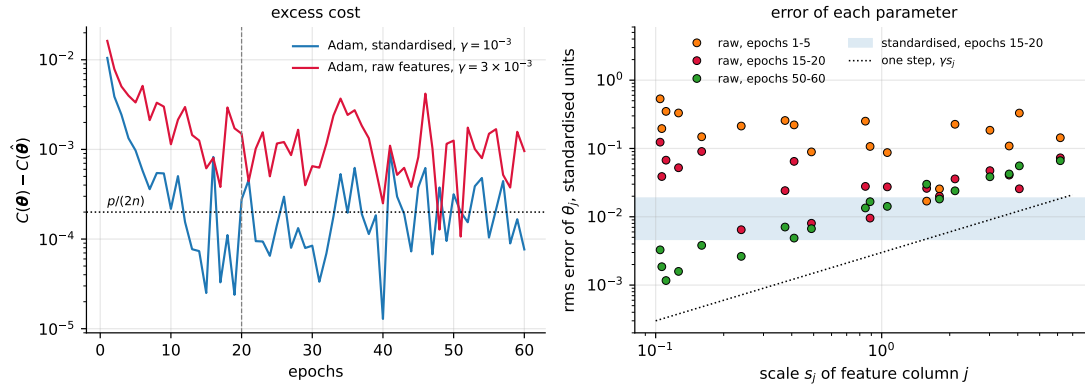
Fig. 5.8 Adam with M = 32 followed for sixty epochs on the standardised features ( \gamma = 10^{-3} ) and on the raw ones ( \gamma = 3 \times 10^{-3} ), the learning rates of Table 5.1. Left: excess cost at the end of each epoch; the dashed line marks the twenty epochs of the table, the dotted line the floor p/(2n) . Right: root-mean-square error of each parameter of the raw run, converted to standardised units, against the scale s_j of its column, over three windows of epochs; the band is the range of the standardised run and the dotted line the length \gamma s_j of one step in these units, Eq. (5.47). The parameters of the small columns arrive late, those of the large columns never stop rattling.
