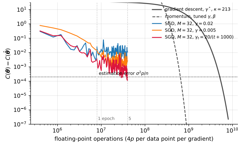
Fig. 4.5 Excess cost against floating-point operations on a least-squares problem with n = 10^5 , p = 20 and \kappa = 213 , from \theta_0 = \mathbf{0} . Full-batch gradient descent at \gamma^* and momentum with tuned parameters against minibatch SGD ( M = 32 ) at two constant learning rates and with the schedule (4.52). The dotted line is the estimation error \sigma^2 p/n of Eq. (4.48); SGD with the schedule is there within five epochs, momentum in 81 full gradients and gradient descent in 640.
