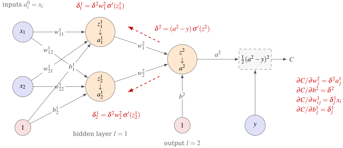
Fig. 8.12 The network of Section 8.8.2: two inputs, one hidden layer of two sigmoid nodes and one output node, nine parameters in all. The weight w_{ij}^1 leaves input i and arrives at hidden node j , as in Fig. 8.6. Red: the backward pass of Eqs. (8.48) and (8.52). The output error \delta^2 travels back along each of the two edges w_j^2 separately, and each hidden node multiplies what arrives by its own \sigma'(z_j^1) ; the gradient of every weight is then the error at the node the weight arrives at times the signal at the node it leaves, Eq. (8.53).
