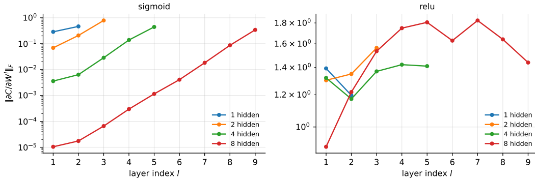
Fig. 8.14 Norm of the weight gradient at each layer after one backward pass, for networks of 1, 2, 4 and 8 hidden layers of 30 units on the digits data. Left: sigmoid activations, showing severe attenuation towards the input. Right: ReLU, which preserves the gradient far better.
