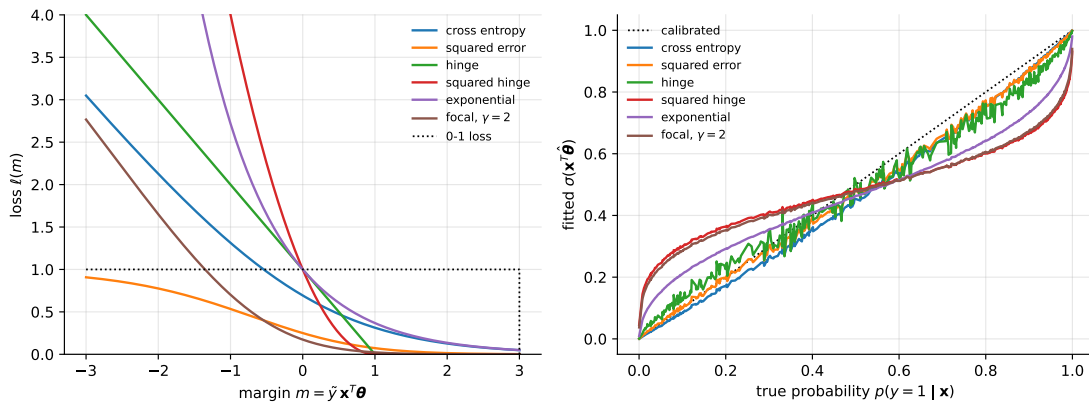
Fig. 5.9 Left: the loss functions of Table 5.2 against the margin, for a point of class \tilde{y} = +1 ; the 0–1 loss is dotted. Right: the probability \sigma(\mathbf{x}^T \hat{\boldsymbol{\theta}}) obtained by minimising each loss with a linear model on 400 points drawn from a true logistic model, plotted against the true probability. The cross entropy and the squared error follow the diagonal; the exponential loss recovers half the log-odds, so its curve is the diagonal compressed towards \frac{1}{2} ; the squared hinge and the focal loss are compressed further; the hinge loss does not estimate a probability at all.
