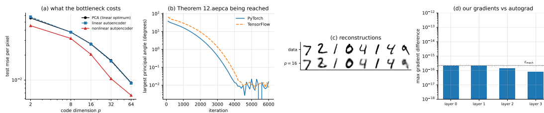
Fig. 12.7 (a) Reconstruction error against code dimension on MNIST, Table 12.2: PCA is the floor for any linear map of that rank, the linear autoencoder tracks it, and the nonlinear one beats it by a margin that grows with p . (b) The largest principal angle between the encoder subspace and the span of the top p eigenvectors, against training iteration, in both frameworks: Theorem 12.5 being reached, not assumed. (c) Test images and their reconstructions at p = 16 . (d) The largest disagreement between our gradients and each framework's, against the double-precision unit roundoff.
