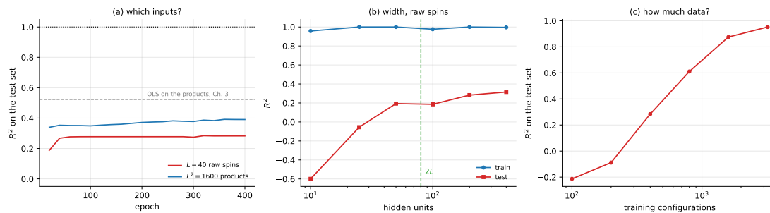
Fig. 8.16 Learning the Ising energy with a one-hidden-layer network. (a) Test R^2 against epoch for the L = 40 raw spins and for the L^2 = 1600 products of Section 3.16, both from 400 training configurations. (b) Width study on the raw spins; the dashed line marks the 2L units that suffice for the exact representation of Proposition 8.8. (c) Test R^2 against the number of training configurations: the limitation is data, not capacity.
