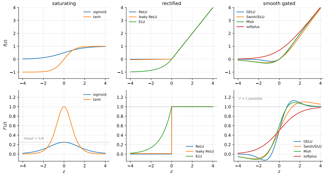
Fig. 8.9 Nine activation functions in three families (top) and their derivatives (bottom). Only the derivative enters the backpropagation recursion (8.66). Dotted lines mark \max \sigma' = 1/4 in the left panel and f' = 1 in the other two.
