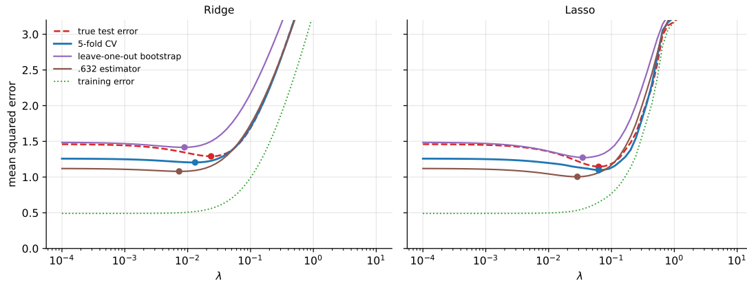
Fig. 3.5 Four estimates of the test error of Ridge (left) and the Lasso (right) along the penalty grid, for the training set of Figure 3.4: the training error, five-fold cross-validation (3.92), the leave-one-out bootstrap (3.98) and the .632 estimator (3.99), with B = 100 replicas per grid point. The dashed curve is the true expected test error. Dots mark the minimum of each curve: the .632 minimum sits to the left of the true one because the estimator inherits 0.368 of the training error, which decreases towards \lambda = 0 .
