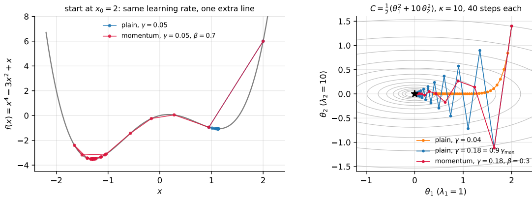
Fig. 4.4 Following the steps of gradient descent with and without momentum. Left: the quartic f(x) = x^4 - 3x^2 + x from x_0 = 2 with \gamma = 0.05 ; plain descent stops in the nearer, shallower minimum, momentum with \beta = 0.7 carries the iterate over the hump into the global one. Right: forty steps on the bowl \frac{1}{2}(\theta_1^2 + 10\theta_2^2) with \kappa = 10 , at a small learning rate, at 0.9 of the stability bound (4.20), and with momentum \beta = 0.3 at the same learning rate.
