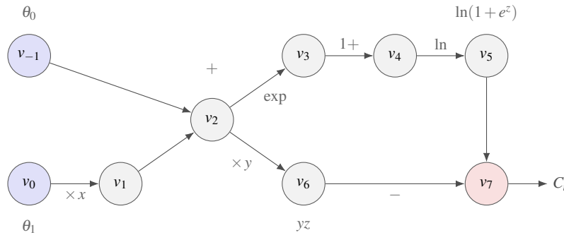
Fig. 5.5 The computational graph of the cross entropy of one observation, trace (5.38). The inputs are the two parameters; the data x and y enter as constants on the edges. The linear predictor z = v_2 fans out into the softplus branch along the top and the label branch along the bottom, and the reverse sweep of Eq. (5.41) sums the two when it reaches v_2 , producing the residual p - y .
