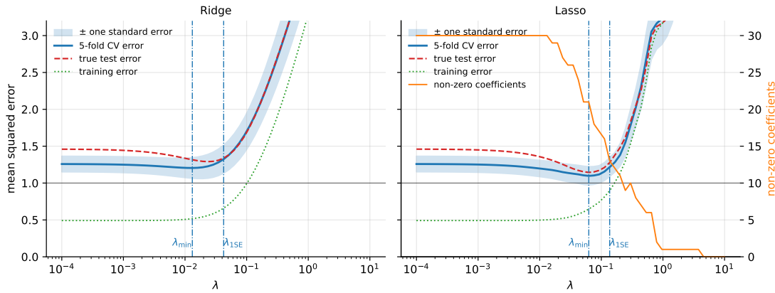
Fig. 3.4 Five-fold cross-validation of Ridge (left) and the Lasso (right) on the sparse problem of the text: n = 100 , p = 30 , correlation 0.7^{|i-j|} , eight non-zero coefficients, \sigma = 1 . The cross-validation error (3.92) is shown with its one-standard-error band (3.93); the dashed curve is the true expected test error of the model refitted at each \lambda , measured on 20000 fresh observations, and the dotted curve the training error. The horizontal line is the noise floor \sigma^2 = 1 . The vertical lines mark \lambda_{\min} of Eq. (3.94) and \lambda_{1SE} of Eq. (3.96); for the Lasso the number of non-zero coefficients is drawn against the right-hand axis.
