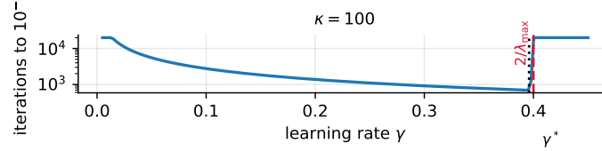
Fig. 4.1 Iterations required to reach an error of 10^{-6} against the learning rate, for a quadratic with eigenvalues \{0.05, 1, 5\} . The optimum lies at \gamma^* and the method diverges beyond 2/\lambda_{\max} , as predicted by Eqs. (4.20) and (4.26).
