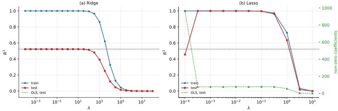
Fig. 3.10 Test and training R^2 against the penalty for the Ising problem, with the OLS test score marked. Ridge (a) needs \lambda \sim 10^3 before anything happens, and never beats OLS. The Lasso (b) has a broad plateau on which it is exact, and the count of non-zero coefficients (right axis, dashed) sits at about 2L = 80 across it.
