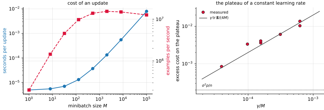
Fig. 4.6 Left: measured time per SGD update and throughput in examples per second against the minibatch size, for the least-squares problem of Fig. 4.5; the update is nearly free up to M \approx 30 , and the throughput saturates near M = 2000 , the two regimes of Eq. (4.56). Right: the excess cost at which SGD with a constant learning rate levels off, for seven combinations of \gamma and M , against the prediction \gamma \text{tr} \mathbf{S} / (4M) of Eq. (4.51); the dotted line is the estimation error \sigma^2 p / n .
