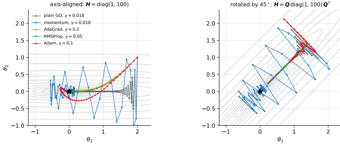
Fig. 4.8 The first hundred steps of five optimisers on the quadratic bowl with Hessian eigenvalues 1 and 100, from the same starting point. Left: the Hessian is diagonal, and the adaptive methods, which rescale each coordinate by its own gradient history, move diagonally towards the minimum while plain gradient descent zigzags down the steep direction and crawls along the flat one. Right: the same bowl rotated by 45^\circ , with the same eigenvalues and condition number. Gradient descent and momentum are unaffected; the adaptive methods, whose diagonal rescaling cannot see the off-diagonal curvature, lose most of their advantage.
