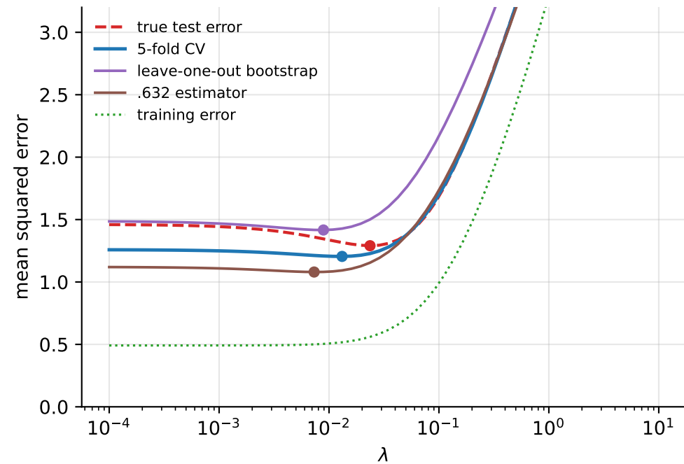
Ridge
