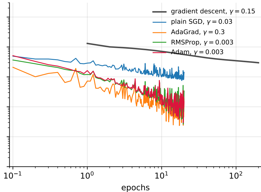
raw features, columns scaled by 10^{\pm 1}
