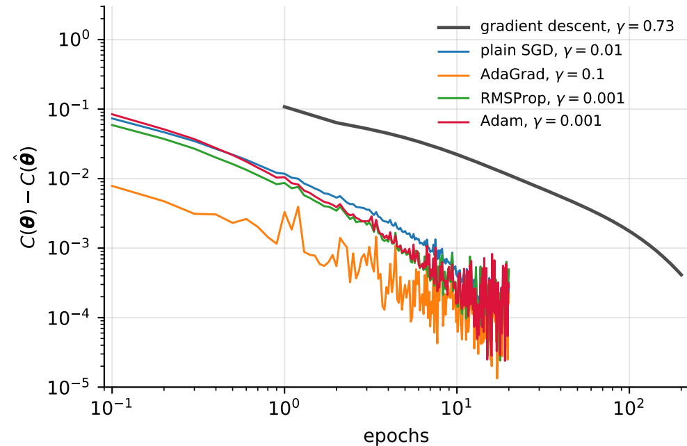
standardised features
