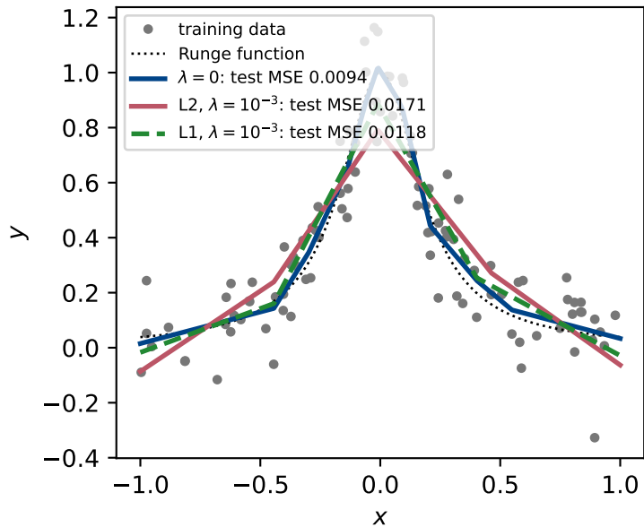
(a) 1-50-1 network, 20000 GD steps
