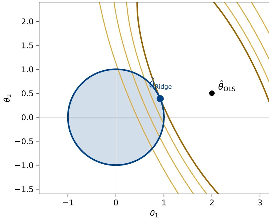
Ridge: \theta_1^2 + \theta_2^2 \leq t (a circle)
