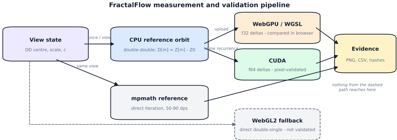
Figure 2: The precision-sensitive reference is computed once on the CPU. WebGPU and CUDA then evaluate the same per-pixel recurrence at different precisions. Direct arbitrary-precision iteration supplies an independent reference rather than reusing the implementation under test.
