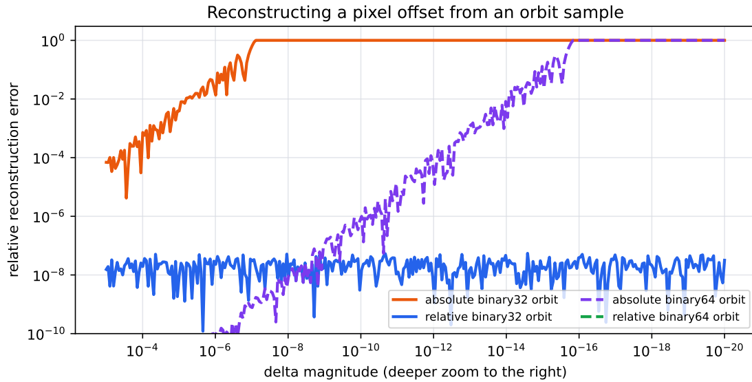
Figure 3: The mechanism, isolated: reconstructing a known pixel offset from an orbit sample stored either absolutely or relative to Z_0 . The absolute form loses the offset entirely once it falls below the local spacing of the format, nine orders of magnitude apart for the two precisions; the relative form holds its relative accuracy however small the offset gets. Controlled arithmetic, not a renderer measurement – Figure 4 is the same effect on real frames.
