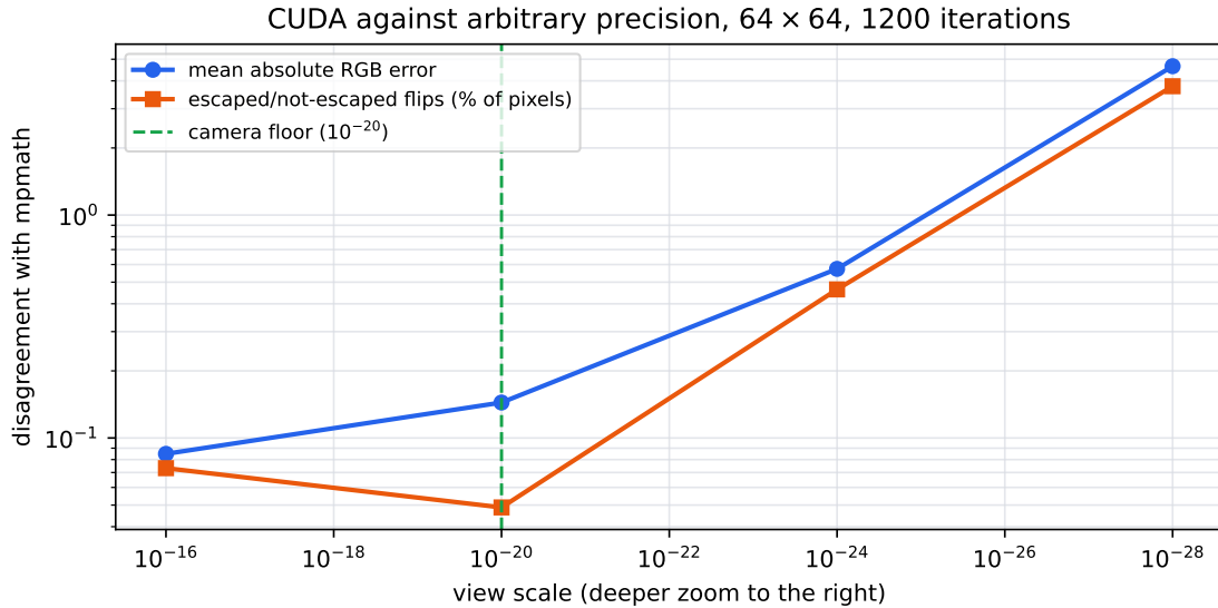
Figure 5: Archived depth sweep. Disagreement with arbitrary precision is flat until 10^{-20} and then climbs by two orders of magnitude over the next eight. The escape flips are palette-independent; the mean is not.
