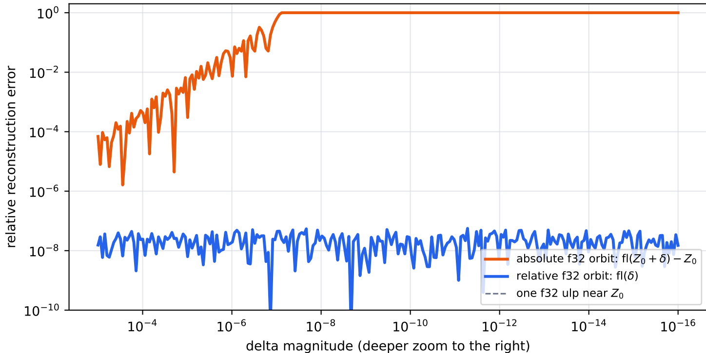
Controlled f32 quantization experiment near a repelling fixed point
