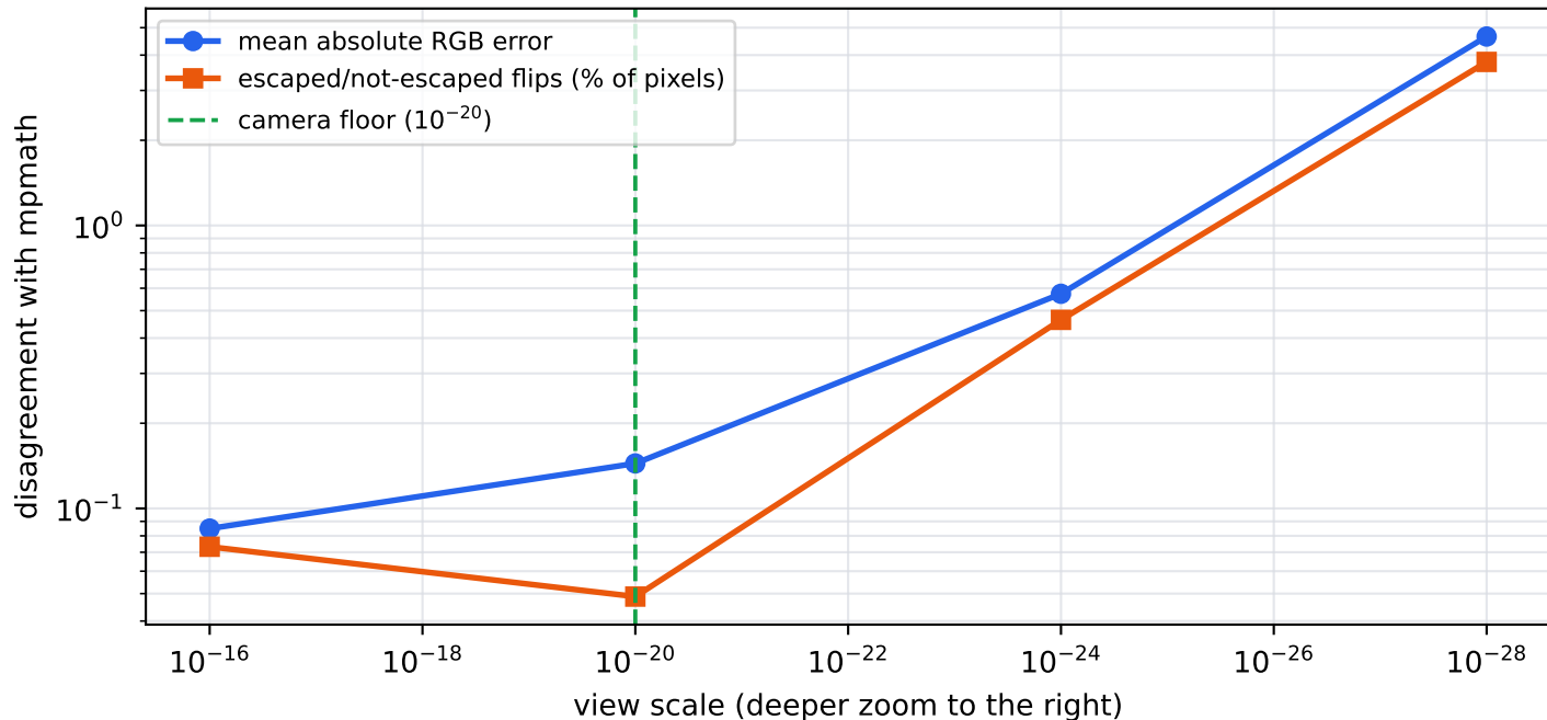
CUDA against arbitrary precision, 64 × 64, 1200 iterations
