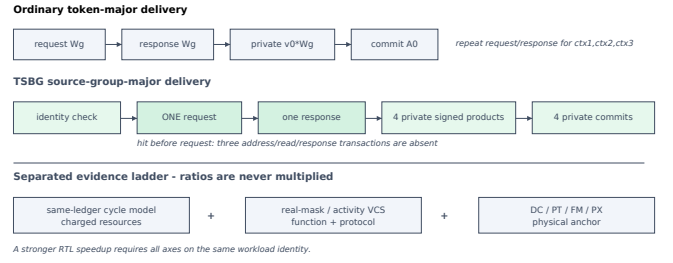
Fig. 2. TSBG suppresses redundant SRAM transactions before request. The lower ladder separates model, VCS, and physical evidence; component ratios from different rungs are not multiplied.
