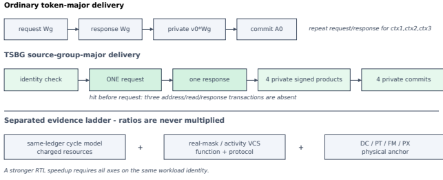
Fig. 2. TSBG suppresses redundant SRAM transactions before request. The lower ladder separates model, VCS, and physical evidence; component ratios from different rungs are not multiplied.
