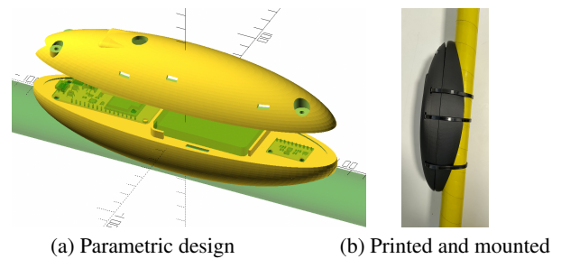
Figure 1: The staff-mounted sensor unit, held on with zip ties so it can be repositioned or removed without marking the staff: (a) the parametric OpenSCAD design; (b) the printed enclosure zip-tied to the bō.
