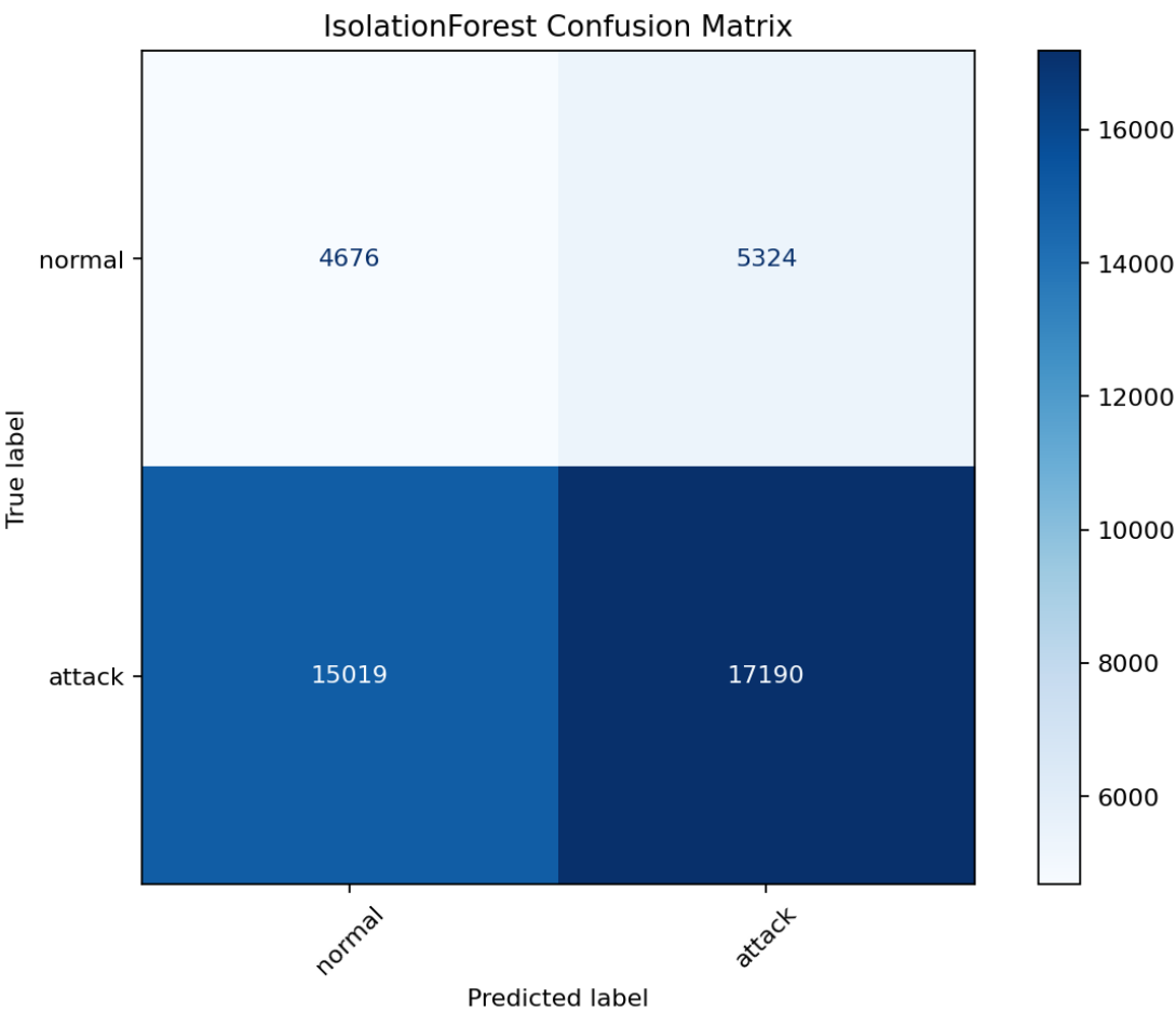
Figure 7.3: IsolationForest Confusion Matrix: Binary anomaly detection (normal vs. attack)
