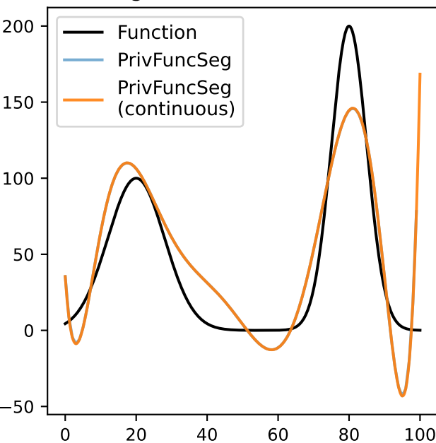
Degree-8 Monomial Basis
