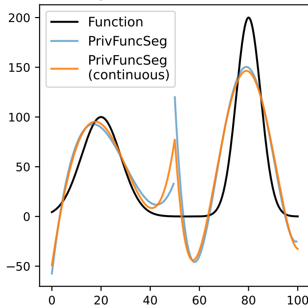
Degree-16 Monomial Basis
