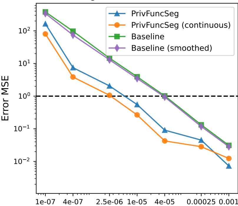
Degree-8 Monomial Basis
