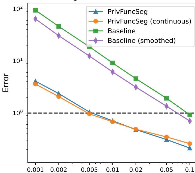
Degree-8 Monomial Basis
