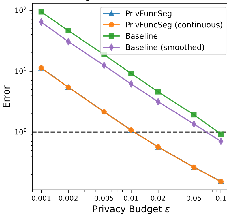
Degree-8 Monomial Basis
