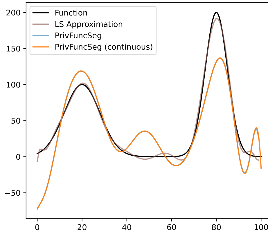
Degree-16 Monomial Basis
