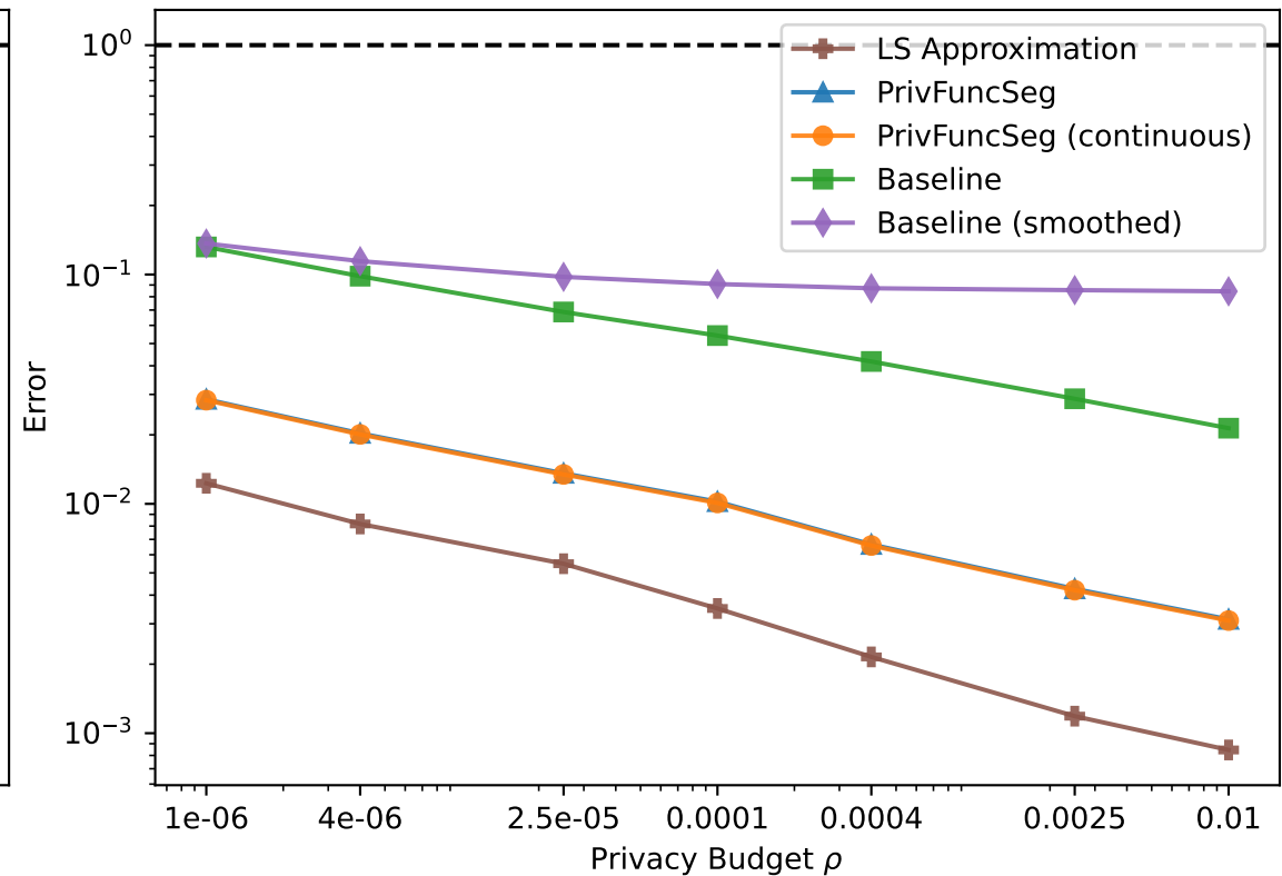
Degree-16 Monomial Basis
