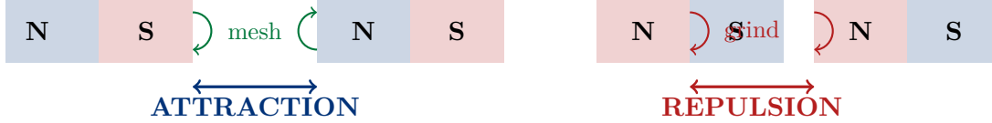
Figure 1.3: Gear synchronization governs magnetic forces. Left: N-S pairing — torsion vectors rotate in complementary directions, the lattice gears mesh, and the objects are drawn together to minimise vacuum stress. Right: N-N pairing — torsion vectors rotate in the same direction, gears grind against each other, and the lattice pressure pushes the objects apart.
