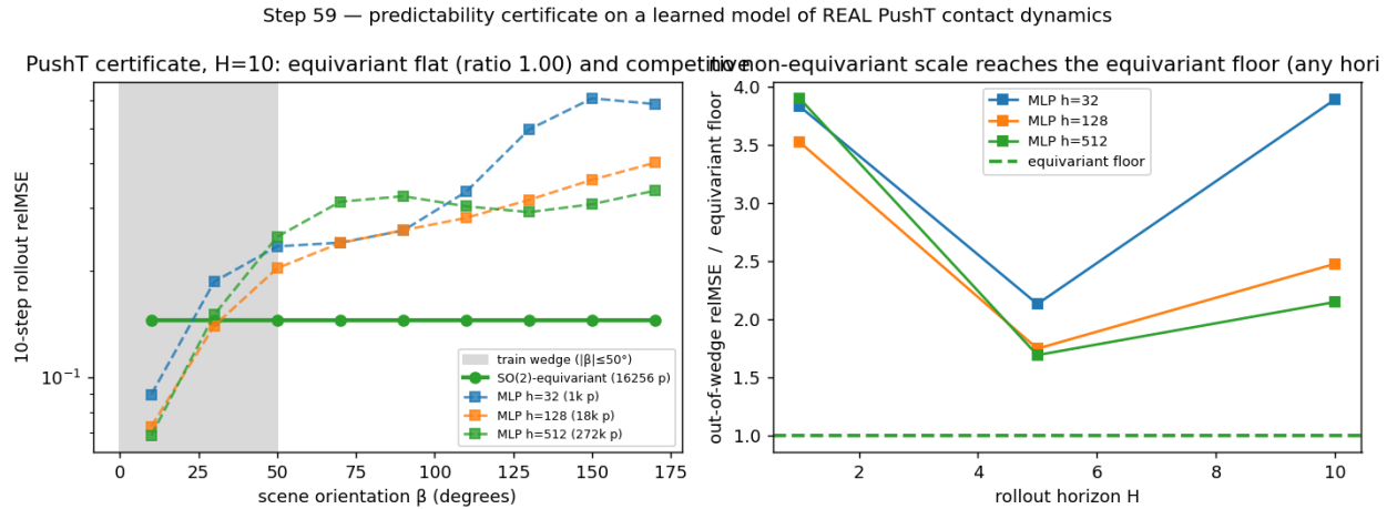
Figure 6: Experiment 9 (PushT, real contact dynamics). Left: 10-step rollout relMSE over the orbit of scene orientations — the learned SO(2)-equivariant model is exactly flat (ratio 1.00) and competitive in-distribution, while non-equivariant baselines dip in-wedge then climb out. Right: across a 160× parameter ladder no baseline reaches the equivariant floor out-of-wedge, at any rollout horizon.
