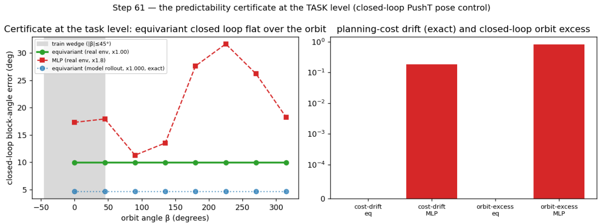
Figure 8: Experiment 11 (the certificate at the task level). Left: closed-loop block-angle error over the orbit of scene orientations — the equivariant model under a G -equivariant planner is exactly flat under model rollout (ratio 1.000) and flat on the real env, while a 4.3\times -larger MLP degrades out of the training wedge. Right: the \text{SO}(2) -invariant planning cost is orbit-invariant to the float floor under the equivariant model and materially distorted under the MLP.
