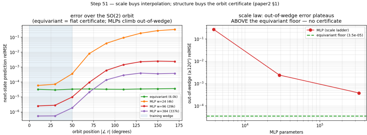
Figure 4: Left: error over the \text{SO}(2) orbit (equivariant flat; the scaled baselines dip below it in-wedge then climb out). Right: out-of-wedge error versus baseline scale plateaus far above the equivariant floor.
