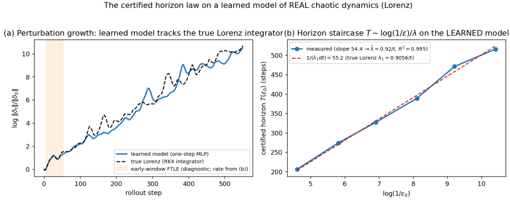
Figure 3: The horizon staircase on a learned model of real chaotic dynamics (E2, Lorenz). Left: the learned one-step model’s perturbation growth tracks the true Lorenz integrator over 550 steps. Right: the certified horizon T(\epsilon_0) on the learned model is linear in \log(1/\epsilon_0) ( R^2=0.995 ), and the measured slope sits on the prediction 1/(\lambda_1 dt) from the textbook Lorenz exponent — Theorem B’s law lifted to a learned model of a genuinely chaotic system (Proposition 7(a)).
