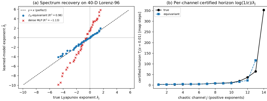
Figure 6: Figure A2. High-dimensional spectral horizon (E2, 40-D Lorenz-96). Left: recovered vs. true Lyapunov exponent for all 40 channels — the \mathbb{Z}_N -equivariant cyclic-conv (blue) lies on y = x ( R^2=0.98 ); the dense MLP (red \times ) is scattered far off ( R^2 = -1.1 ). Right: per-channel certified horizon \log(1/\epsilon)/\lambda_j : the equivariant model tracks the truth across the spectrum. Structure recovers the high-dimensional spectral horizon a dense model of equal data cannot.
