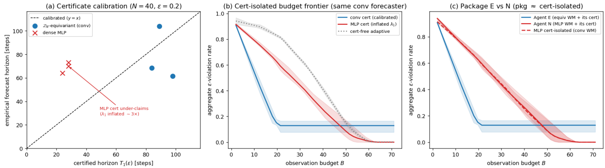
Figure 21: Experiment 22 — structure \rightarrow a trustworthy certificate \rightarrow a budgeted re-observation decision (40-D Lorenz-96, 3 seeds). (a) Certificate calibration: the \mathbb{Z}_N -equivariant model lies on the measured-vs-certified-horizon diagonal; the dense baseline’s certificate under-claims the horizon (its \lambda_1 is inflated \sim 3\times ). (b) Cert-isolated budget frontier (same equivariant forecaster throughout): timing re-observation by the equivariant certificate (blue) reaches low aggregate violation at \sim 1/3 the observation budget the inflated baseline certificate (red) needs; a certificate-free adaptive scheduler (grey) only catches up at \sim 3\times the budget. (c) Package end-to-end — the baseline-forecaster agent (red solid) tracks the cert-isolated baseline (red dashed), confirming the gap is the certificate, not the forecaster. Bands min–max over seeds.
