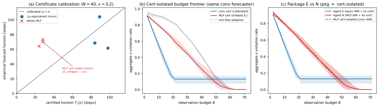
Figure 23: Experiment 22 — structure \rightarrow a trustworthy certificate \rightarrow a budgeted re-observation decision (40-D Lorenz-96, 3 seeds). (a) Certificate calibration: the \mathbb{Z}_N -equivariant model lies on the measured-vs-certified-horizon diagonal; the dense baseline’s certificate under-claims the horizon (its \lambda_1 is inflated \sim 3\times ). (b) Cert-isolated budget frontier (same equivariant forecaster throughout): timing re-observation by the equivariant certificate (blue) reaches low aggregate violation at \sim 1/3 the observation budget the inflated baseline certificate (red) needs; a certificate-free adaptive scheduler (grey) only catches up at \sim 3\times the budget. (c) Package end-to-end — the baseline-forecaster agent (red solid) tracks the cert-isolated baseline (red dashed), confirming the gap is the certificate, not the forecaster. Bands min–max over seeds.
