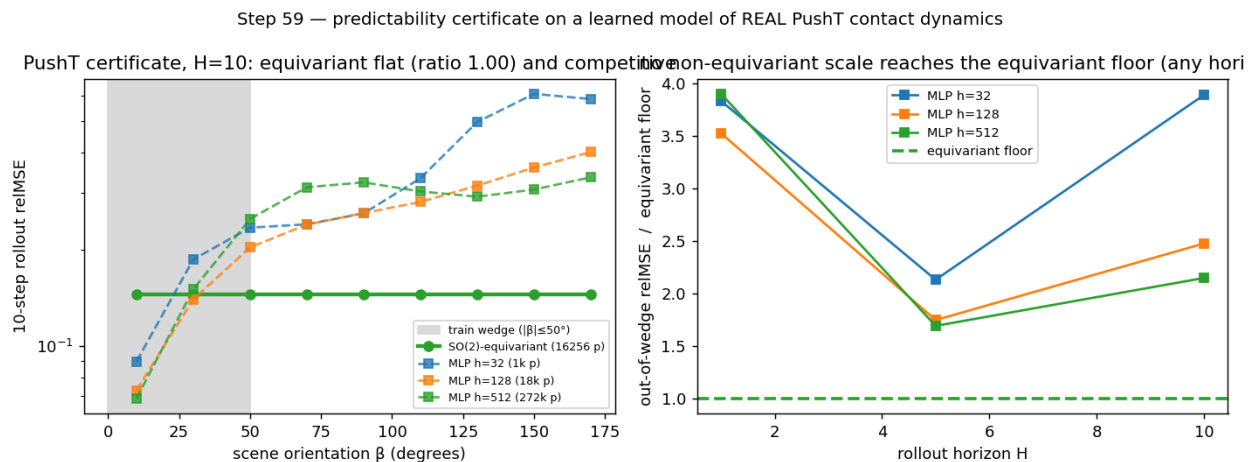
Figure 7: Experiment 9 (PushT, real contact dynamics). Left: 10-step rollout relMSE over the orbit of scene orientations — the learned SO(2) -equivariant model is exactly flat (ratio 1.00) and competitive in-distribution, while non-equivariant baselines dip in-wedge then climb out. Right: across a 160\times parameter ladder no baseline reaches the equivariant floor out-of-wedge, at any rollout horizon.
