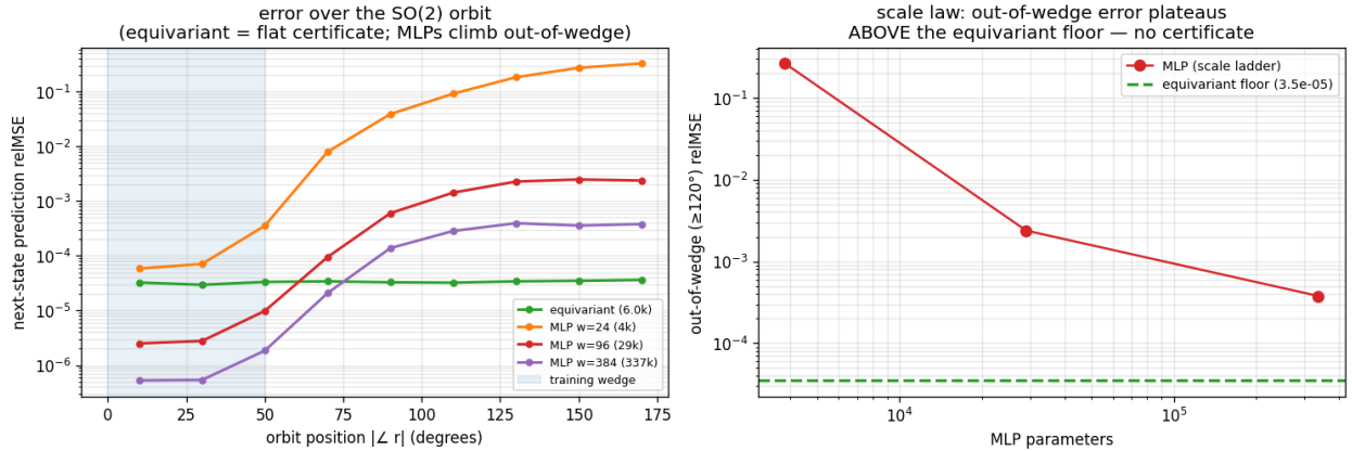
Figure 5: Left: error over the SO(2) orbit (equivariant flat; the scaled baselines dip below it in-wedge then climb out). Right: out-of-wedge error versus baseline scale plateaus far above the equivariant floor.
