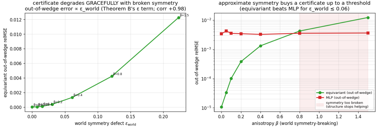
Figure 5: Left: equivariant out-of-wedge error grows \propto \epsilon_{\text{world}} (Theorem B’s \epsilon term). Right: the equivariant model beats the baseline out-of-wedge up to a symmetry-content threshold, then crosses over.
