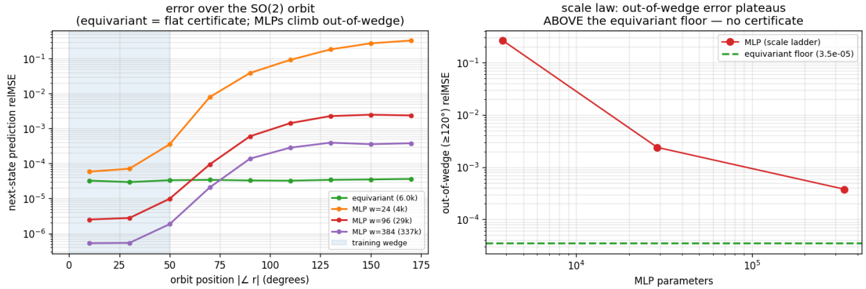
Figure 4: Step 51 — left: error over the SO(2) orbit (equivariant flat; MLPs dip below it in-wedge then climb out); right: out-of-wedge error vs MLP scale plateaus far above the equivariant floor.
