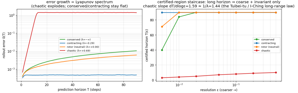
Figure 3: The horizon \times resolution staircase (E2). The measured certified horizon per channel as the demanded resolution \epsilon sharpens, recovering T_j(\epsilon) \sim \log(1/\epsilon)/\lambda_j (slope 1.3–1.6): chaotic channels are certified to a few steps, slow/invariant channels to dozens.
