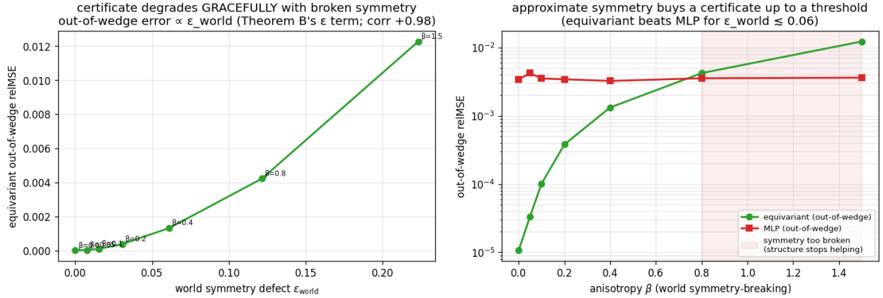
Step 53 — approximate symmetry: graceful certificate degradation (paper2 §6 / Theorem B)
