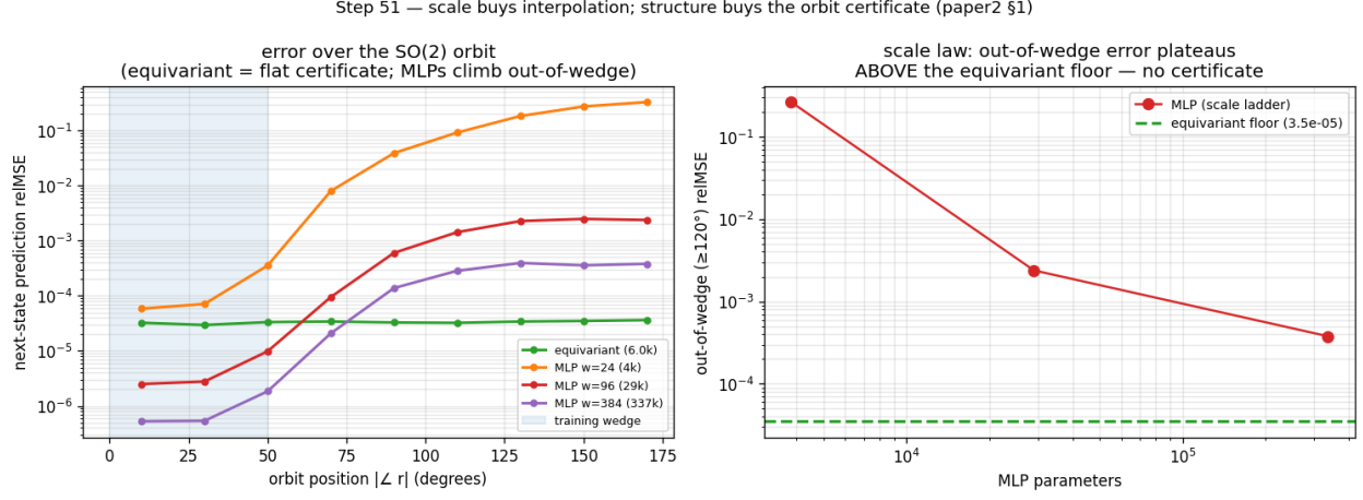
Figure 4: Step 51 — left: error over the SO(2) orbit (equivariant flat; MLPs dip below it in-wedge then climb out); right: out-of-wedge error vs MLP scale plateaus far above the equivariant floor.
