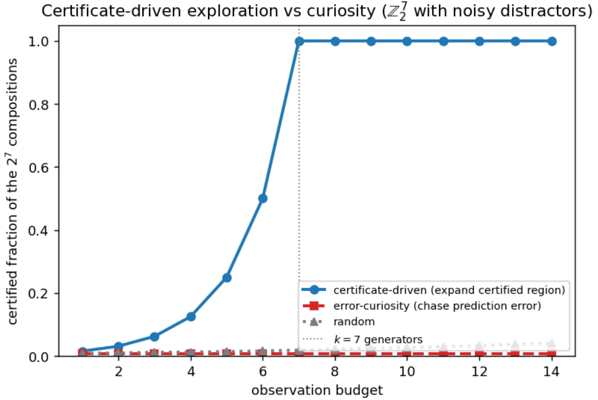
Figure 8: Certificate-driven active inference (E8). On a \mathbb{Z}_2^7 compositional world with noisy distractor actions, an explorer that maximizes the certified region certifies all 128 compositions in exactly 7 observations (the generator basis), while a prediction-error-curiosity explorer is lured by the high-error distractors and certifies almost nothing at the same budget.
