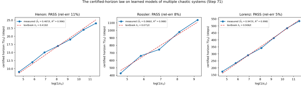
Figure 5: Figure A2. The certified-horizon law across a class of learned chaotic models (E2). The identical learned-model staircase on a 2D map (Hénon), a small-exponent flow (Rössler), and a large-exponent flow (Lorenz) is linear in \log(1/\epsilon_0) and its slope (blue) recovers the textbook exponent (red dashed). The law is a property of chaotic dynamics, not of Lorenz; the residual bias is decomposed by Proposition 8.
