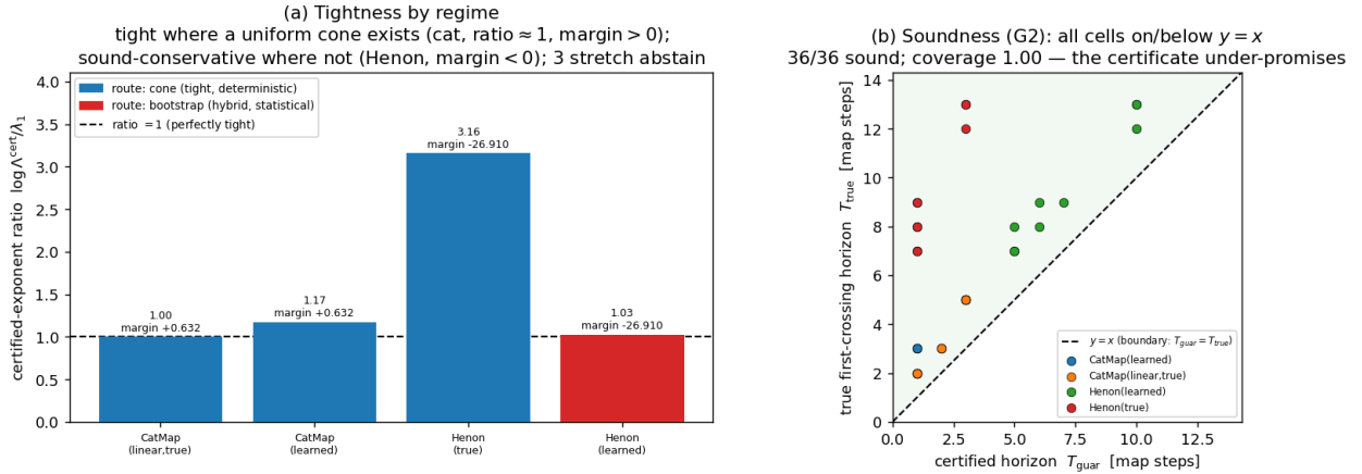
Figure 21: Experiment 20 — a certified horizon read from the learned model (step82). Left : per-system certified-exponent / true- \lambda_1 ratio, colored by route — the cone certificate is tight (ratio \approx 1 ) on uniformly-hyperbolic dynamics (cat map, incl. a learned net and a nonlinear Anosov perturbation) and soundly conservative on Hénon, where its cone-margin diagnostic goes negative and it abstains to a bootstrap horizon. Right : soundness — T_{\text{guar}} vs. T_{\text{true}} across all (system, seed, \epsilon ): every certified horizon lies on or below y = x (it never over-promises). A tight a-priori certificate is achievable exactly where uniform hyperbolicity holds, and the certificate knows which regime it is in.
