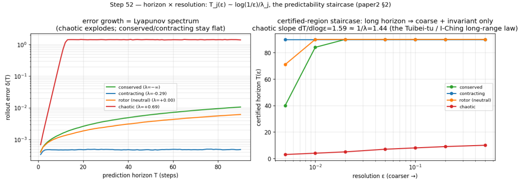
Figure 6: Figure A3. The horizon \times resolution staircase on a controlled spectrum (E2). The measured certified horizon per channel as the demanded resolution \epsilon sharpens, recovering T_j(\epsilon) \sim \log(1/\epsilon)/\lambda_j (slope 1.3–1.6): chaotic channels are certified to a few steps, slow/invariant channels to dozens.
