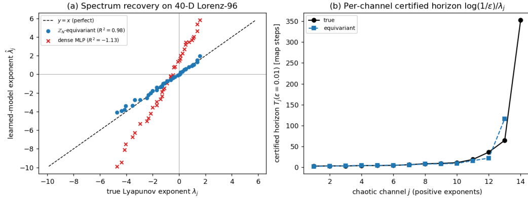
Figure 5: Figure A2. High-dimensional spectral horizon (E2, 40-D Lorenz-96). Left: recovered vs. true Lyapunov exponent for all 40 channels — the \mathbb{Z}_N -equivariant cyclic-conv (blue) lies on y = x ( R^2 = 0.98 ); the dense MLP (red \times ) is scattered far off ( R^2 = -1.1 ). Right: per-channel certified horizon \log(1/\epsilon)/\lambda_j : the equivariant model tracks the truth across the spectrum. Structure recovers the high-dimensional spectral horizon a dense model of equal data cannot.
