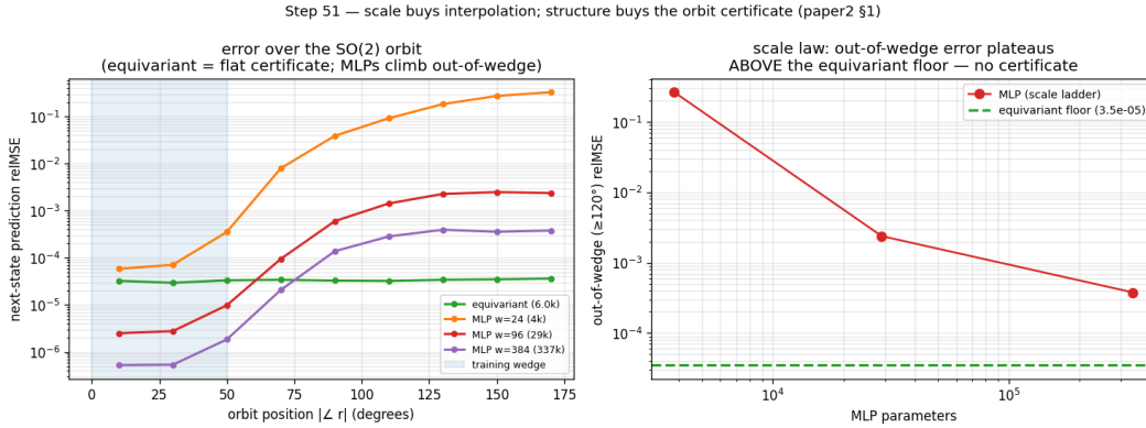
Figure 8: Structure versus scale (E4). The equivariant model is orbit-flat (a certificate); an 88×-scaled non-equivariant model buys in-distribution interpolation (it beats the equivariant model inside the training wedge) but its error climbs 10–155× above the equivariant floor out of the wedge — scale buys interpolation, not the certificate.
