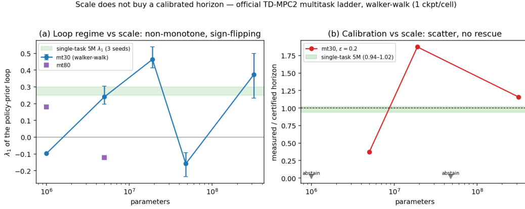
Figure 6: Figure A3. Scale does not buy a calibrated horizon (E14). (a) \lambda_1 of the walker-walk policy-prior loop across the official multitask ladder: sign-flipping, non-monotone (contracting at 1M and 48M). (b) Calibration at \epsilon=0.2 : scatter across sizes; no multitask scale reaches the single-task 5M band (0.94–1.02, green).
