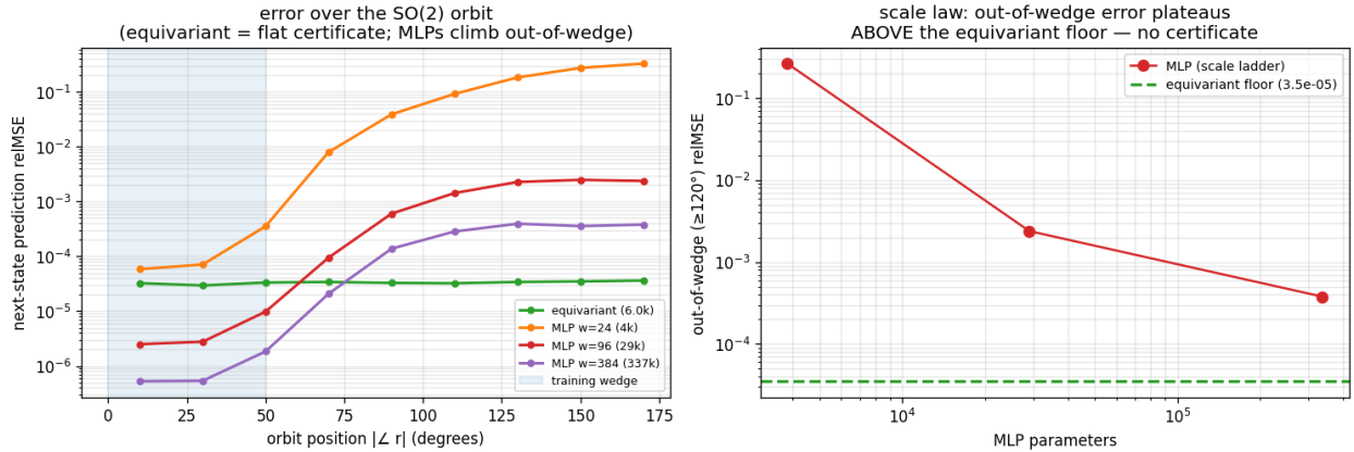
Figure 4: Left: error over the SO(2) orbit (equivariant flat; the scaled baselines dip below it in-wedge then climb out). Right: out-of-wedge error versus baseline scale plateaus far above the equivariant floor.
