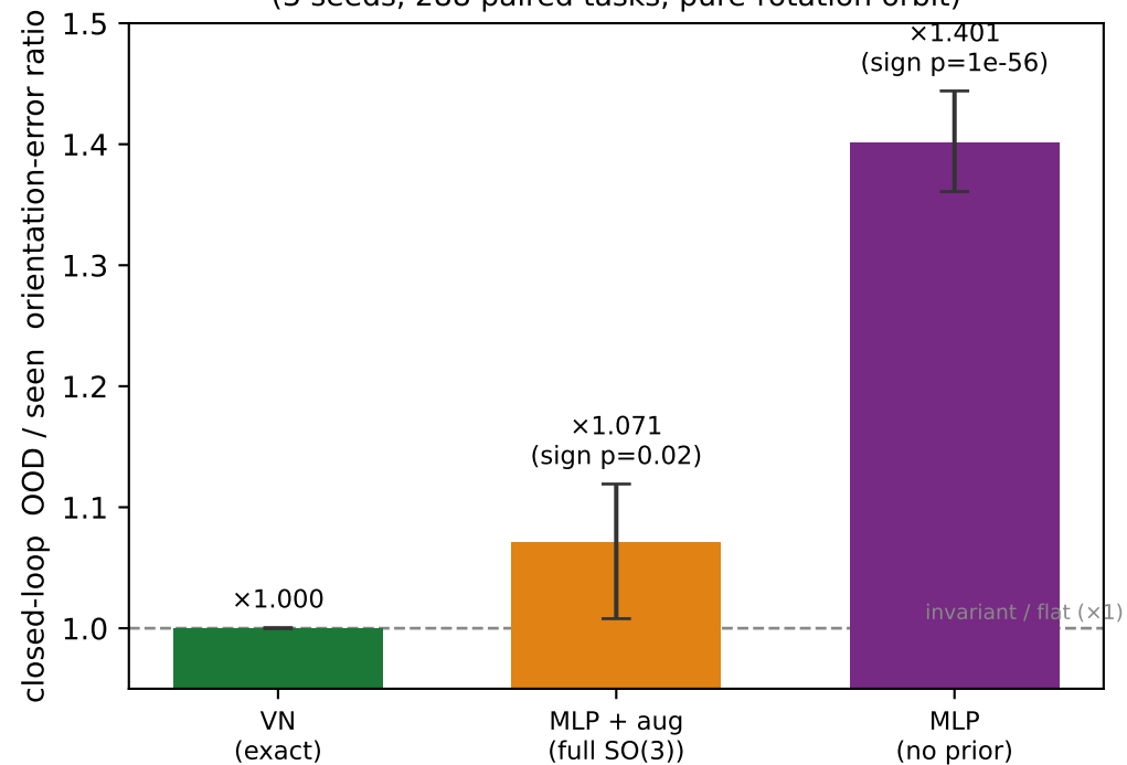
(a) Only the exact model closes the loop (3 seeds, 288 paired tasks, pure-rotation orbit)
