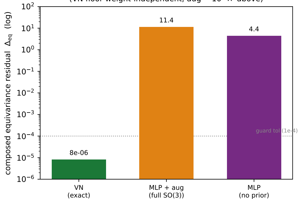
(b) Augmentation never approximates equivariance (VN floor weight-independent; aug \sim 10^6 \times above)
