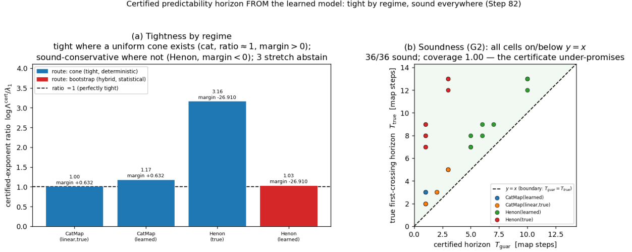
Figure 21: Experiment 20 — a certified horizon read from the learned model (step82). Left : per-system certified-exponent / true- \lambda_1 ratio, colored by route — the cone certificate is tight (ratio \approx 1 ) on uniformly-hyperbolic dynamics (cat map, incl. a learned net and a nonlinear Anosov perturbation) and soundly conservative on Hénon, where its cone-margin diagnostic goes negative and it abstains to a bootstrap horizon. Right : soundness — T_{\text{guar}} vs. T_{\text{true}} across all (system, seed, \epsilon ): every certified horizon lies on or below y = x (it never over-promises). A tight a-priori certificate is achievable exactly where uniform hyperbolicity holds, and the certificate knows which regime it is in.
