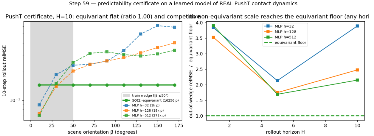
Figure 8: Experiment 9 (PushT, real contact dynamics). Left: 10-step rollout relMSE over the orbit of scene orientations — the learned SO(2)-equivariant model is exactly flat (ratio 1.00) and competitive in-distribution, while non-equivariant baselines dip in-wedge then climb out. Right: across a 160 \times parameter ladder no baseline reaches the equivariant floor out-of-wedge, at any rollout horizon.
