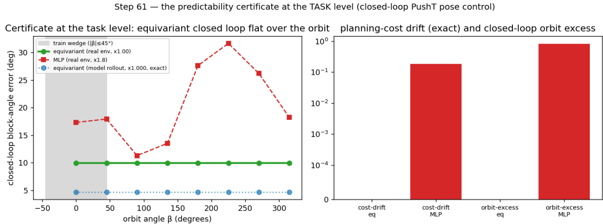
Figure 10: Experiment 11 (the certificate at the task level). Left: closed-loop block-angle error over the orbit of scene orientations — the equivariant model under a G -equivariant planner is exactly flat under model rollout (ratio 1.000) and flat on the real env, while a 4.3 \times -larger MLP degrades out of the training wedge. Right: the SO(2) -invariant planning cost is orbit-invariant to the float floor under the equivariant model and materially distorted under the MLP.
