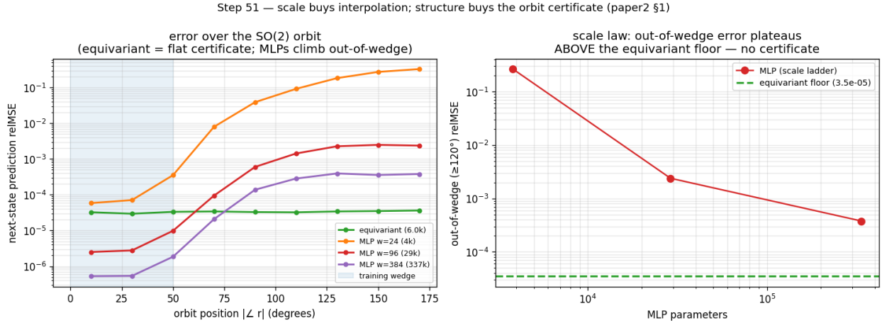
Figure 6: Left: error over the \text{SO}(2) orbit (equivariant flat; the scaled baselines dip below it in-wedge then climb out). Right: out-of-wedge error versus baseline scale plateaus far above the equivariant floor.
