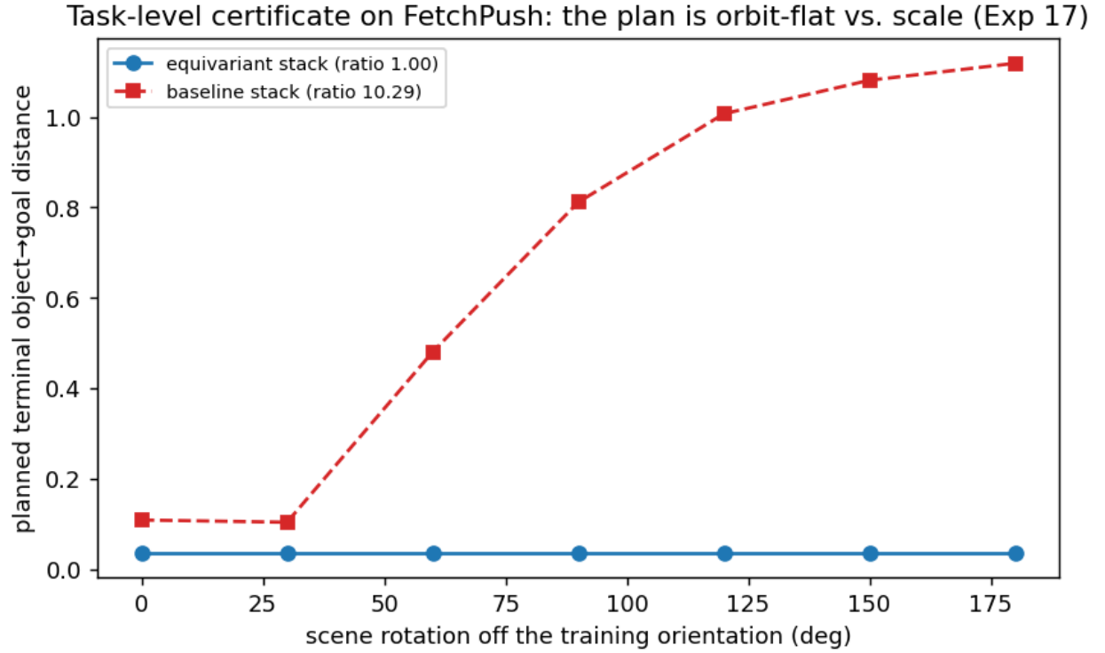
Figure 16: Experiment 17 (the task-level certificate on FetchPush, seed 0; the other seeds match). Planned terminal object→goal distance vs. scene rotation off the training orientation. The equivariant planning stack (blue; equivariant WM + equivariant goal-readout + G -equivariant CEM) produces an exactly orbit-flat plan (ratio 1.000); the scaled-baseline stack (red dashed) degrades 4–10× out of the training orientation. The whole planner is SO(2) -equivariant by construction (proven to the float floor in a unit test), so closed-loop behaviour is orbit-invariant — Theorem A carried through the planner.
