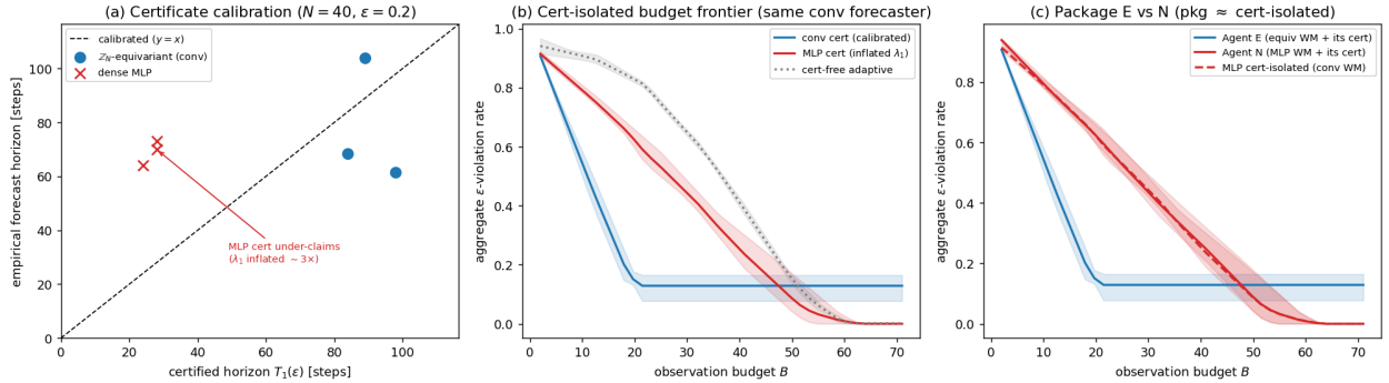
Figure 23: Experiment 22 — structure \rightarrow a trustworthy certificate \rightarrow a budgeted re-observation decision (40-D Lorenz-96, 3 seeds). (a) Certificate calibration: the \mathbb{Z}_N -equivariant model lies on the measured-vs-certified-horizon diagonal; the dense baseline’s certificate under-claims the horizon (its \lambda_1 is inflated \sim 3\times ). (b) Cert-isolated budget frontier (same equivariant forecaster throughout): timing re-observation by the equivariant certificate (blue) reaches low aggregate violation at \sim 1/3 the observation budget the inflated baseline certificate (red) needs; a certificate-free adaptive scheduler (grey) only catches up at \sim 3\times the budget. (c) Package end-to-end — the baseline-forecaster agent (red solid) tracks the cert-isolated baseline (red dashed), confirming the gap is the certificate, not the forecaster. Bands min–max over seeds.
