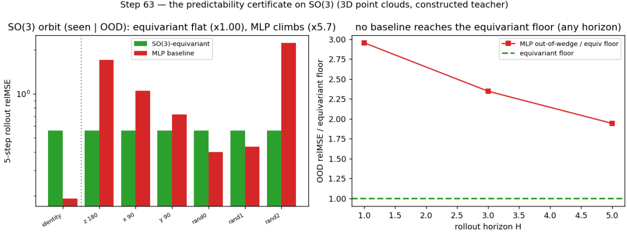
Figure 11: Experiment 12 (the certificate on SO(3) , 3D point clouds, constructed teacher). Left: 5-step rollout relMSE over the SO(3) orbit (in-wedge identity | out-of-distribution rotations) — the learned equivariant model is exactly flat (ratio 1.000) while the 7.4×-larger MLP climbs out of the wedge. Right: across rollout horizon the MLP’s out-of-wedge error stays at or above the equivariant floor, but the gap is modest because the small equivariant model’s floor is high (the “flat is not good” caveat in 3D).
