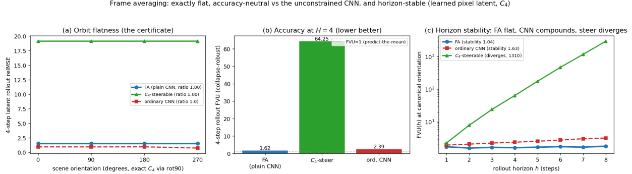
Figure 12: Experiment 13 (the certificate on rendered pixels, C_4 ). (a) 4-step latent-rollout relMSE over the orbit of scene orientations: the frame-averaged model is flat to the float floor (ratio 1.000); the ordinary CNN is also orbit-flat (PushT’s pixel stream is approximately C_4 -symmetric, the augmentation regime of §5.8). (b) Collapse-robust accuracy (FVU) at the canonical orientation: frame averaging matches/beats the unconstrained CNN and is far better than the steerable incumbent (dotted line = predict-the-mean). (c) FVU vs. rollout horizon (log scale): the steerable rollout diverges while the frame-averaged model stays stable . Absolute FVU > 1 for all models is an architecture-agnostic JEPA-latent property, not an equivariance cost.
