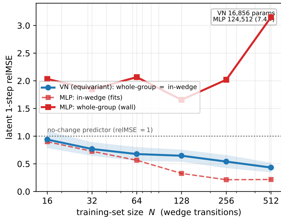
Sample-efficiency frontier (exact SO(3) )
