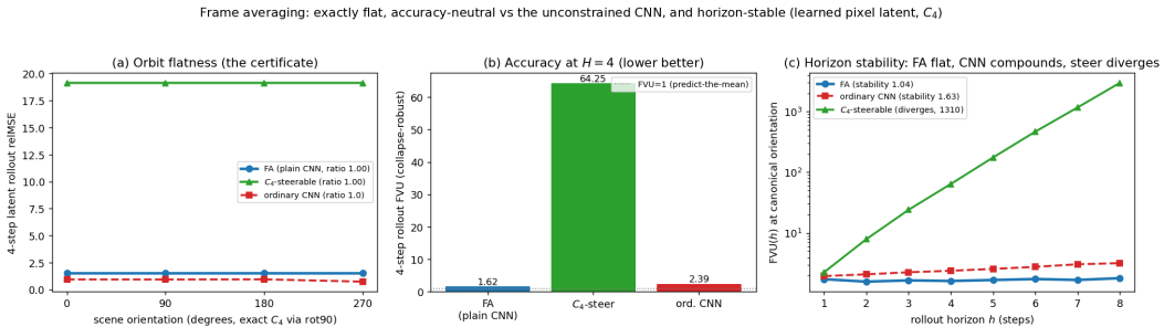
Figure 8: Figure A4. The certificate on raw pixels at no accuracy cost (E6). On rendered PushT frames (exact C_4 ), frame averaging makes a plain CNN/MLP exactly C_4 -equivariant: the latent rollout is flat over the orbit (left, the certificate), it matches or beats an unconstrained CNN on a collapse-robust accuracy metric (centre), and its rollout error stays bounded over horizon while the steerable baseline diverges (right, log scale).
