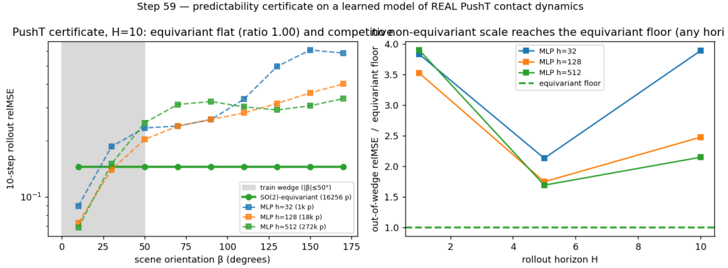
Figure 4: The certificate on real contact dynamics (E5). On PushT (a physics engine we did not author), a learned SO(2)-equivariant world model’s multi-step rollout error is flat over the orbit of scene orientations to the floating-point floor, while a 160× parameter sweep of non-equivariant baselines never reaches the equivariant floor out of distribution.
