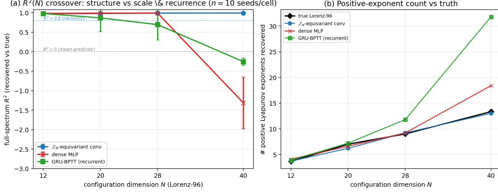
Figure 4: Figure A1. Full-spectrum Lyapunov R^2 vs. N : the \mathbb{Z}_N -conv holds while dense MLP and GRU collapse at N=40 — a phase transition, not a single- N artifact (step83).
