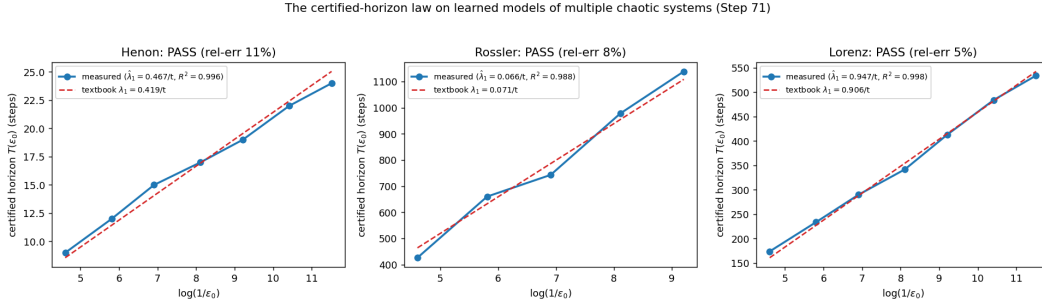
Figure 5: Figure A2. The certified-horizon law across a class of learned chaotic models (E2). The identical learned-model staircase on a 2D map (Hénon), a small-exponent flow (Rössler), and a large-exponent flow (Lorenz) is linear in \log(1/\epsilon_0) and its slope (blue) recovers the textbook exponent (red dashed). The law is a property of chaotic dynamics, not of Lorenz; the residual bias is decomposed by Proposition 8.
