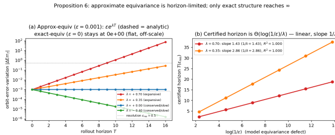
Figure 3: Proposition 6, numerically (the central claim). Left: orbit-error-variation of an \epsilon=10^{-3} -approximately-equivariant model (markers) equals the analytic \epsilon e^{\lambda T} (dashed) to relative error 10^{-14} – 10^{-13} , 3 seeds; an exactly equivariant model sits at the machine-precision floor; \lambda \leq 0 channels stay bounded (infinite horizon). Right: certified horizon linear in \log(1/\epsilon) with slope exactly 1/\lambda ( R^2=1.000 ) — the \Theta(\log(1/\epsilon)/\lambda) law (step65).
