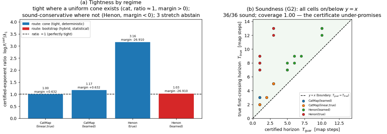
Figure 19: Experiment 20 — a certified horizon read from the learned model (step82). Left: per-system certified-exponent / true- \lambda_1 ratio, colored by route — the cone certificate is tight (ratio \approx 1 ) on uniformly-hyperbolic dynamics (cat map, incl. a learned net and a nonlinear Anosov perturbation) and soundly conservative on Hénon, where its cone-margin diagnostic goes negative and it abstains to a bootstrap horizon. Right: soundness — T_{\text{guar}} vs. T_{\text{true}} across all (system, seed, \epsilon ): every certified horizon lies on or below y = x (it never over-promises). A tight a-priori certificate is achievable exactly where uniform hyperbolicity holds, and the certificate knows which regime it is in.
