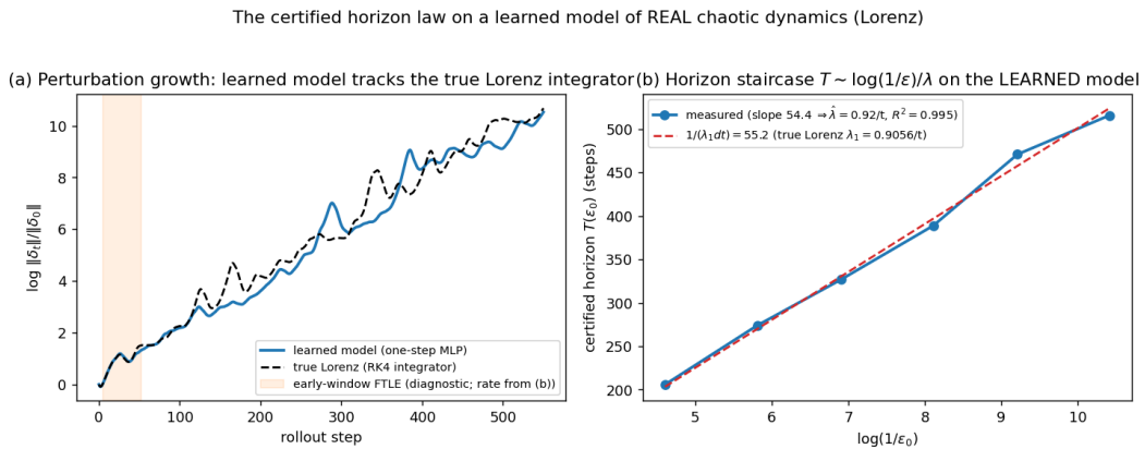
Figure 12: The horizon staircase on a learned model of real chaotic dynamics (E2, Lorenz). Left: the learned one-step model’s perturbation growth tracks the true Lorenz integrator over 550 steps. Right: the certified horizon T(\epsilon_0) on the learned model is linear in \log(1/\epsilon_0) ( R^2=0.995 ), and the measured slope sits on the prediction 1/(\lambda_1 dt) from the textbook Lorenz exponent — Theorem B’s law lifted to a learned model of a genuinely chaotic system (Proposition 7(a)).
