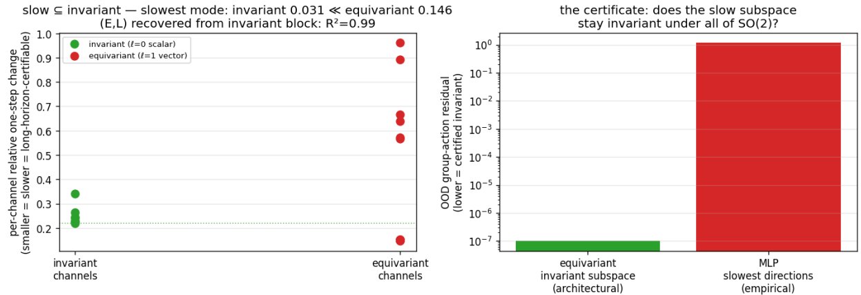
Step 50 — Noether hinge: a learned equivariant model’s slow channels are its invariant ones (paper2 §3)
