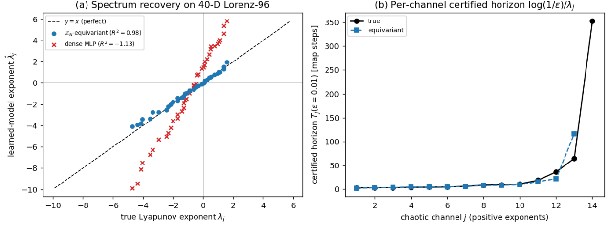
Figure 16: Experiment 18 (the high-dimensional spectral horizon law, N=40 Lorenz-96, seed 0; the other seeds match). (a) Recovered vs. true Lyapunov exponent for all 40 channels: the \mathbb{Z}_N -equivariant cyclic-conv (blue) lies on y = x ( R^2=0.98 ); the dense MLP (red \times ) is scattered far off ( R^2 = -1.1 ), over-amplifying the spectrum. (b) Per-channel certified horizon T_j(\epsilon=0.01) = \log(1/\epsilon)/\lambda_j across the positive exponents: the equivariant model (blue) tracks the truth (black) — short horizons ( \sim few steps) for the most chaotic channels, long ( \sim 350 steps) for the weakly chaotic ones. Structure recovers the spectral stratification a dense model of equal data cannot.
