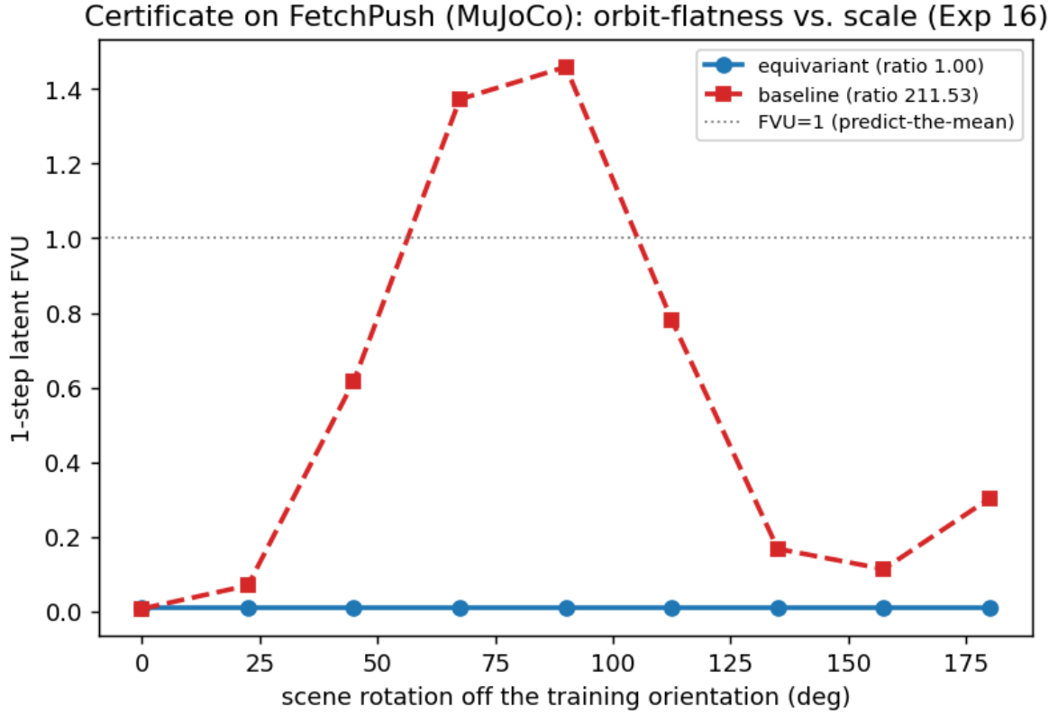
Figure 14: Experiment 16 (the certificate on FetchPush / MuJoCo, seed 0; the other seeds match). One-step latent FVU as the scene is rotated off the single training orientation. The equivariant world model (blue) is exactly orbit-flat (ratio 1.000); the \sim 7\times -larger unconstrained baseline (red dashed) degrades by orders of magnitude out of the training orientation, exceeding predict-the-mean ( FVU = 1 , dotted) near a quarter-turn — yet it interpolates the training orientation competitively. Structure buys the certificate; scale buys only interpolation.
