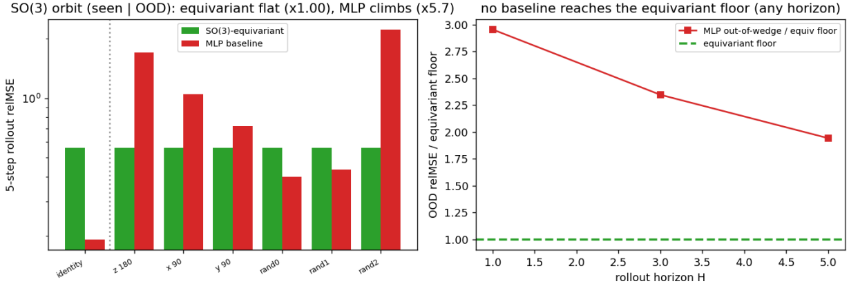
Figure 10: Experiment 12 (the certificate on SO(3), 3D point clouds, constructed teacher). Left: 5-step rollout relMSE over the SO(3) orbit (in-wedge identity | out-of-distribution rotations) — the learned equivariant model is exactly flat (ratio 1.000) while the 7.4×-larger MLP climbs out of the wedge. Right: across rollout horizon the MLP’s out-of-wedge error stays at or above the equivariant floor, but the gap is modest because the small equivariant model’s floor is high (the “flat is not good” caveat in 3D).
