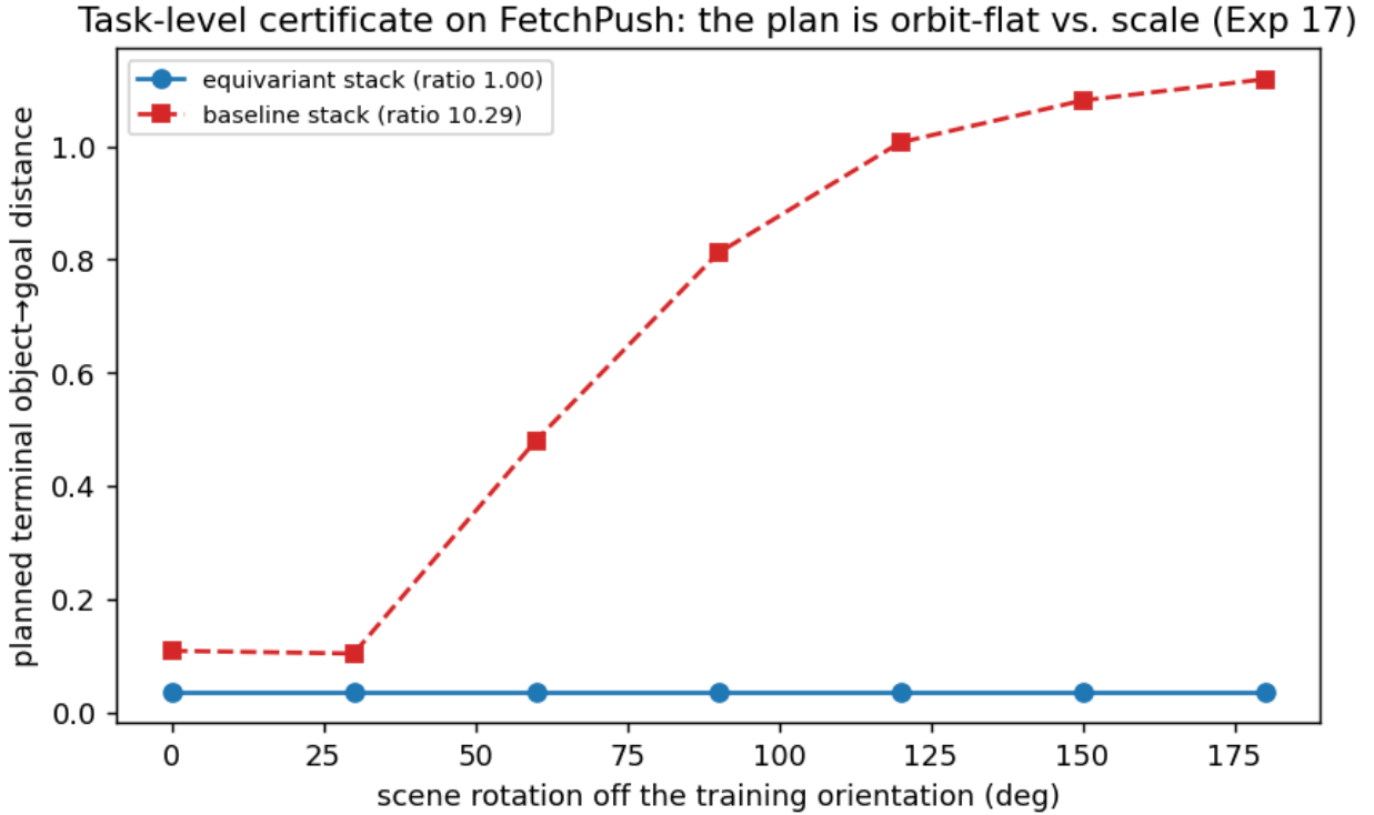
Figure 15: Experiment 17 (the task-level certificate on FetchPush, seed 0; the other seeds match). Planned terminal object→goal distance vs. scene rotation off the training orientation. The equivariant planning stack (blue; equivariant WM + equivariant goal-readout + G -equivariant CEM) produces an exactly orbit-flat plan (ratio 1.000); the scaled-baseline stack (red dashed) degrades 4–10× out of the training orientation. The whole planner is SO(2) -equivariant by construction (proven to the float floor in a unit test), so closed-loop behaviour is orbit-invariant — Theorem A carried through the planner.
