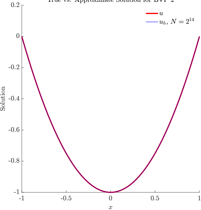
True vs. Approximate Solution for BVP 2
