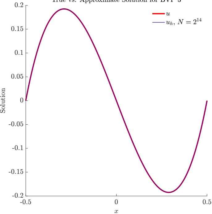
True vs. Approximate Solution for BVP 3
