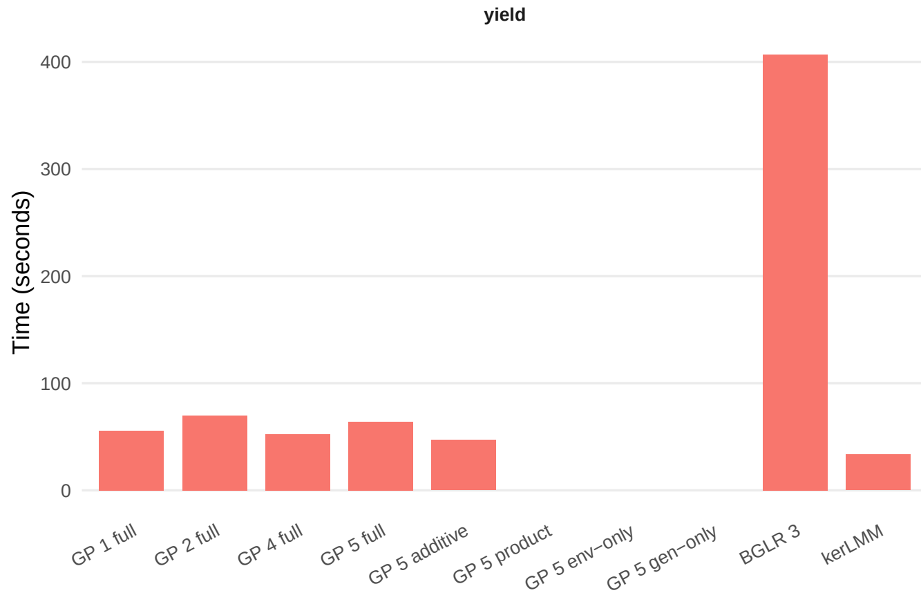
Computation time by model (setup 1, leakage no)
