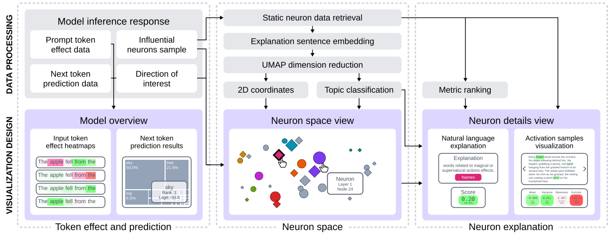
Figure 4.1 Data processing and visualization design of NeuronautLLM.
