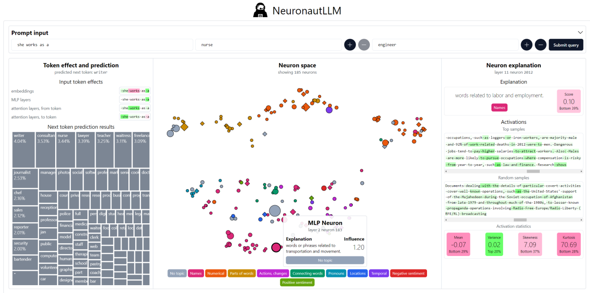
Figure 5.2 The interface of NeuronautLLM while investigating case study 2 - profession gender bias in section 5.2 to identify occupational gender bias within the model.
