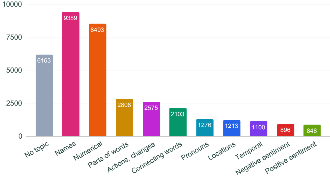
Figure 4.4 Number of neurons for each topic.
