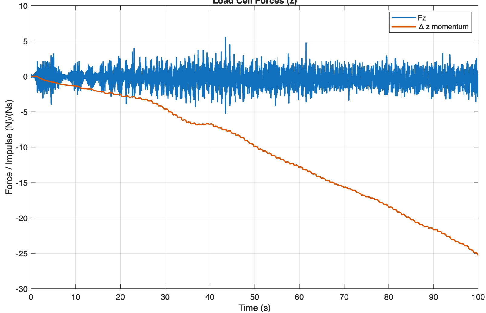
Load Cell Forces (z)
